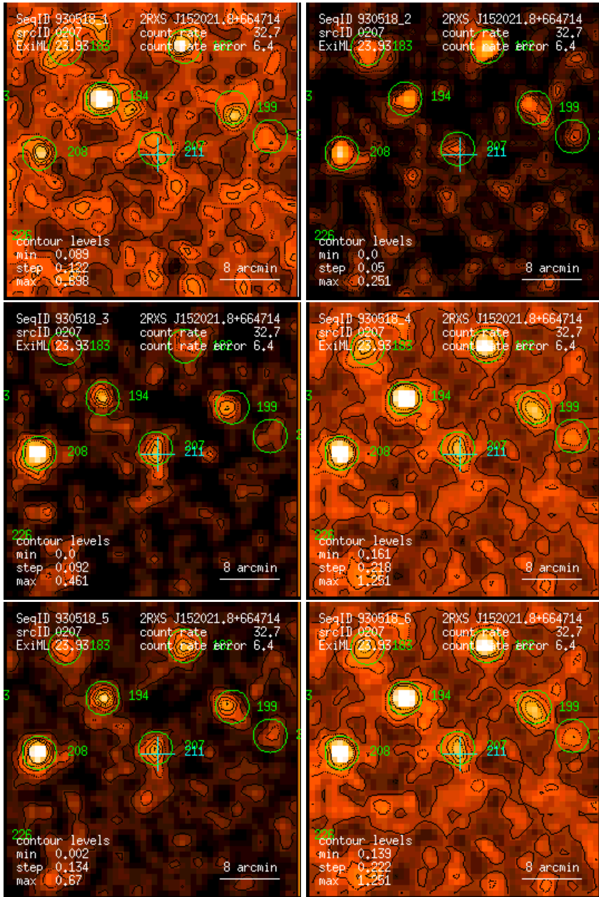
Figure 207: RASS 930518: detection 0207: band rate images, Gaussian filter: (1) PSPC channels 11 – 41, (2) 52 – 90, (3) 91 – 201, (4) 11 – 235, (5) 52 – 201, (6) 11 – 201. Broad band rates in counts/ks. Band rate contour levels in counts/ks/arcmin 2 .
