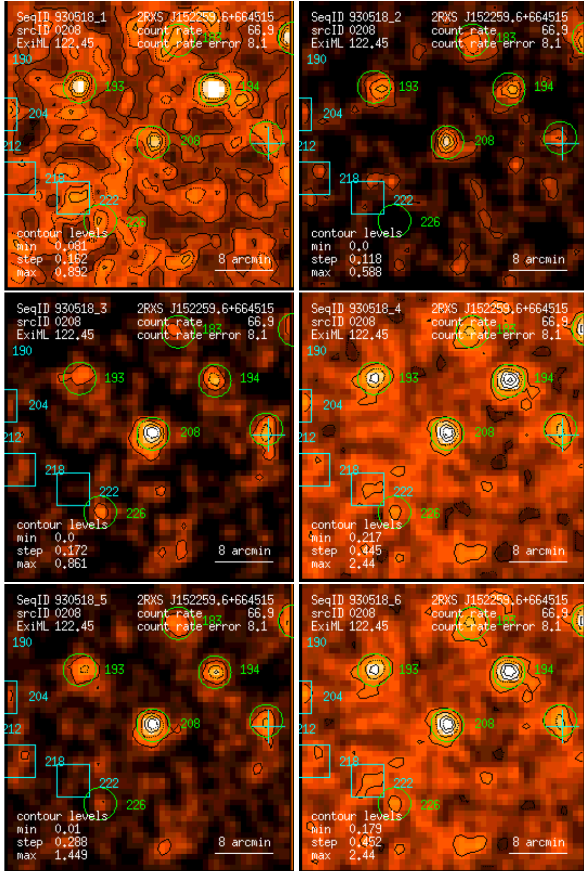
Figure 208: RASS 930518: detection 0208: band rate images, Gaussian filter: (1) PSPC channels 11 – 41, (2) 52 – 90, (3) 91 – 201, (4) 11 – 235, (5) 52 – 201, (6) 11 – 201. Broad band rates in counts/ks. Band rate contour levels in counts/ks/arcmin 2 .
