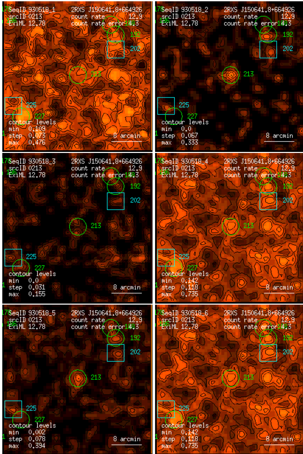
Figure 213: RASS 930518: detection 0213: band rate images, Gaussian filter: (1) PSPC channels 11 – 41, (2) 52 – 90, (3) 91 – 201, (4) 11 – 235, (5) 52 – 201, (6) 11 – 201. Broad band rates in counts/ks. Band rate contour levels in counts/ks/arcmin 2 .
