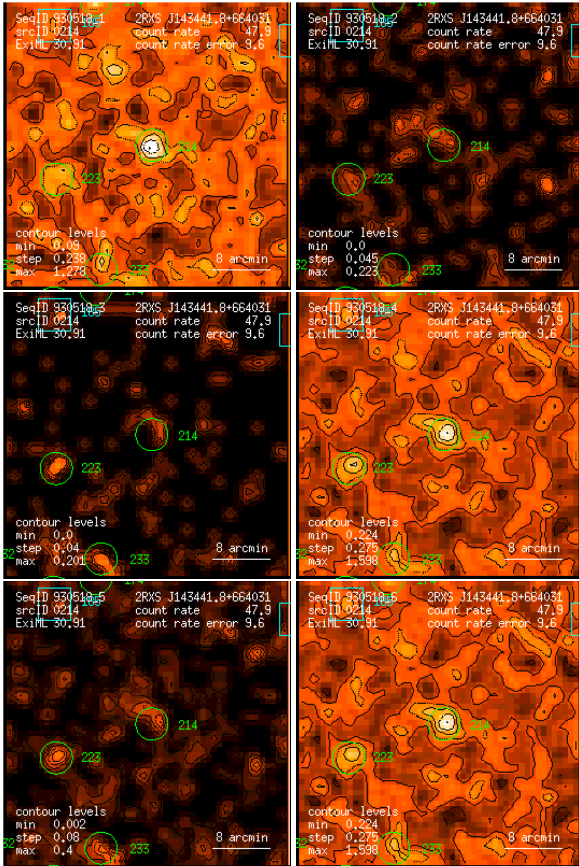
Figure 214: RASS 930518: detection 0214: band rate images, Gaussian filter: (1) PSPC channels 11 – 41, (2) 52 – 90, (3) 91 – 201, (4) 11 – 235, (5) 52 – 201, (6) 11 – 201. Broad band rates in counts/ks. Band rate contour levels in counts/ks/arcmin 2 .
