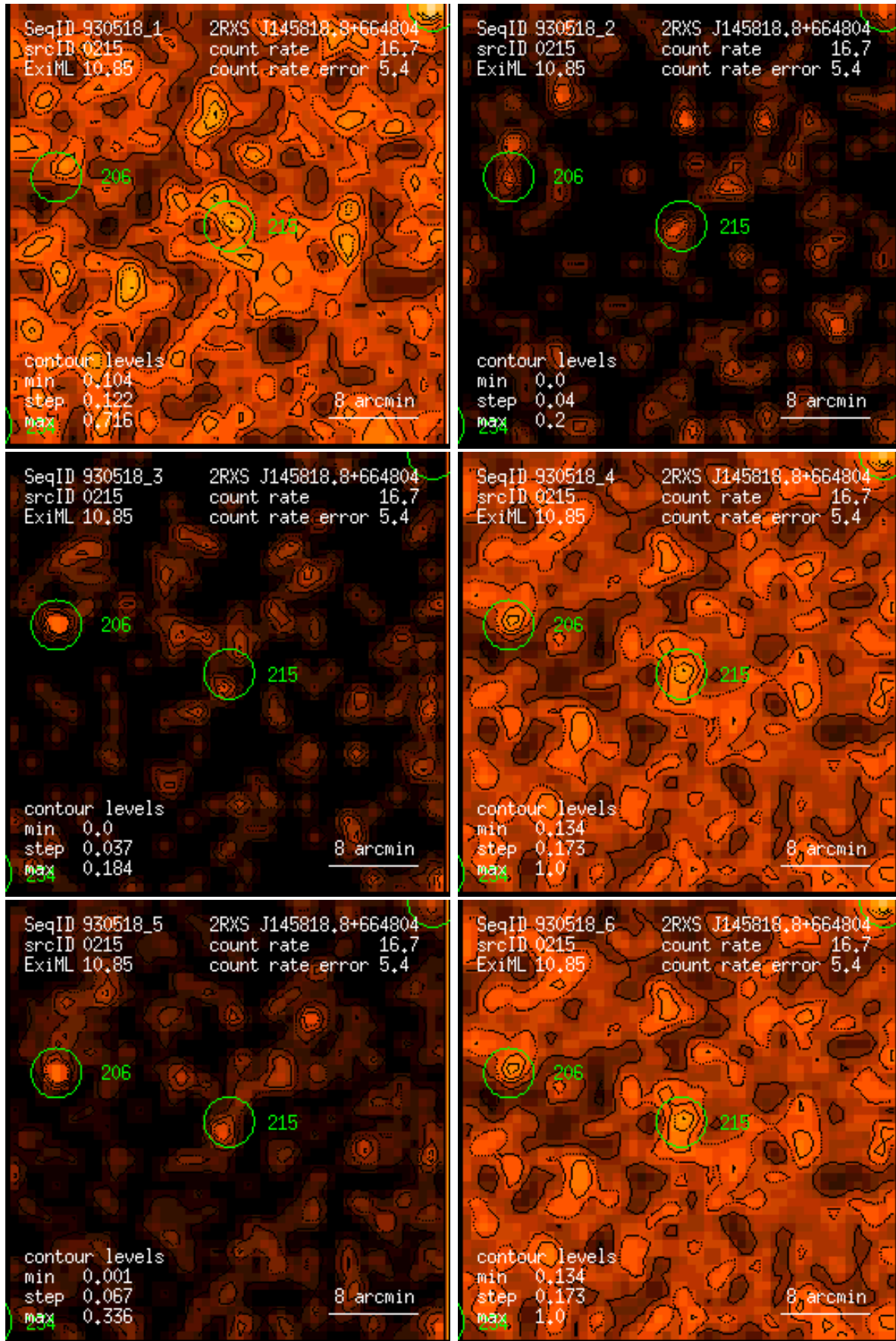
Figure 215: RASS 930518: detection 0215: band rate images, Gaussian filter: (1) PSPC channels 11 – 41, (2) 52 – 90, (3) 91 – 201, (4) 11 – 235, (5) 52 – 201, (6) 11 – 201. Broad band rates in counts/ks. Band rate contour levels in counts/ks/arcmin 2 .
