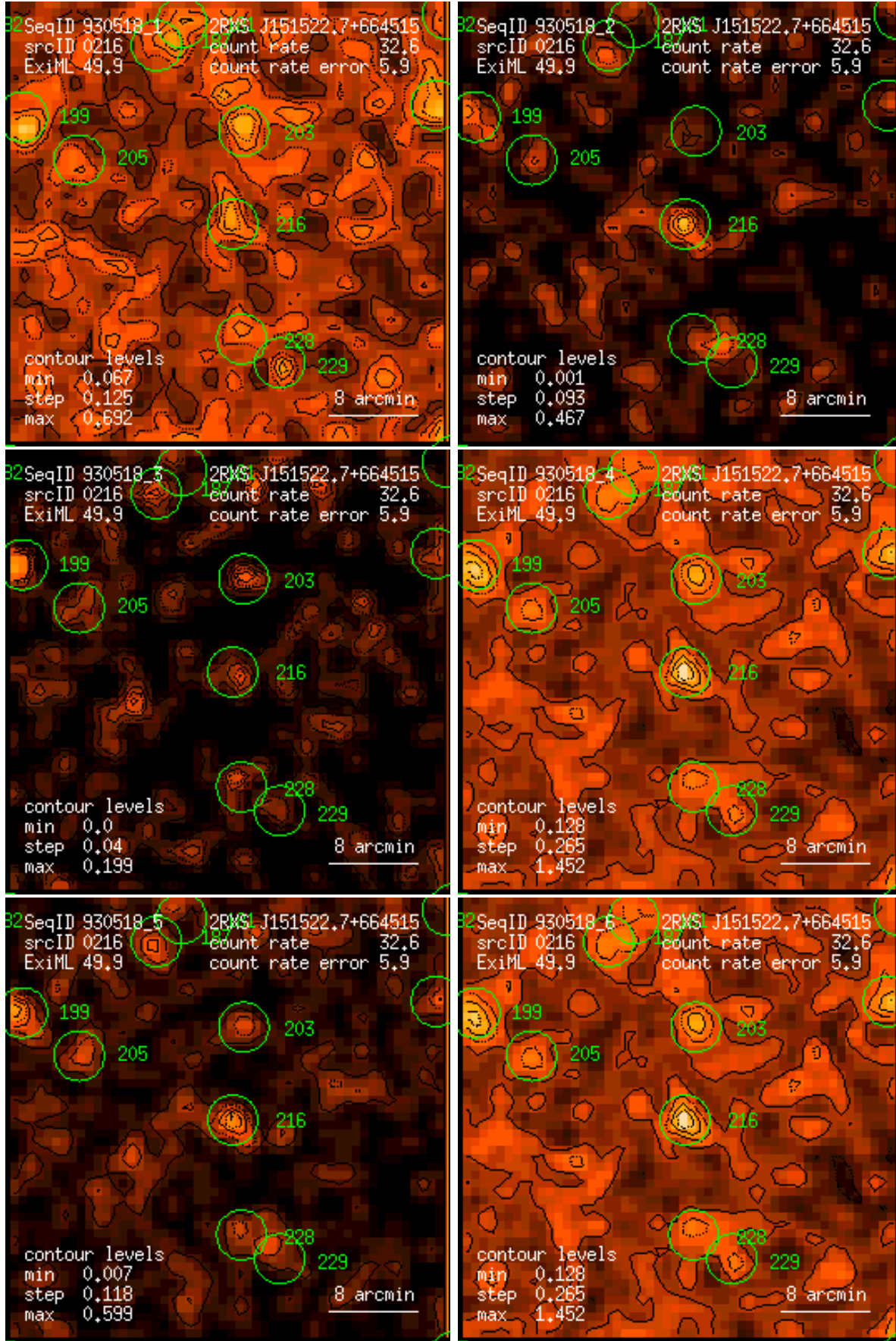
Figure 216: RASS 930518: detection 0216: band rate images, Gaussian filter: (1) PSPC channels 11 – 41, (2) 52 – 90, (3) 91 – 201, (4) 11 – 235, (5) 52 – 201, (6) 11 – 201. Broad band rates in counts/ks. Band rate contour levels in counts/ks/arcmin 2 .
