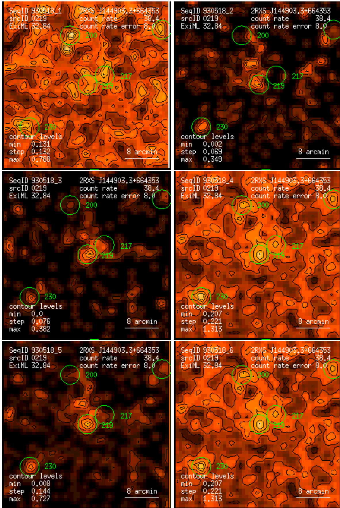
Figure 219: RASS 930518: detection 0219: band rate images, Gaussian filter: (1) PSPC channels 11 – 41, (2) 52 – 90, (3) 91 – 201, (4) 11 – 235, (5) 52 – 201, (6) 11 – 201. Broad band rates in counts/ks. Band rate contour levels in counts/ks/arcmin 2 .
