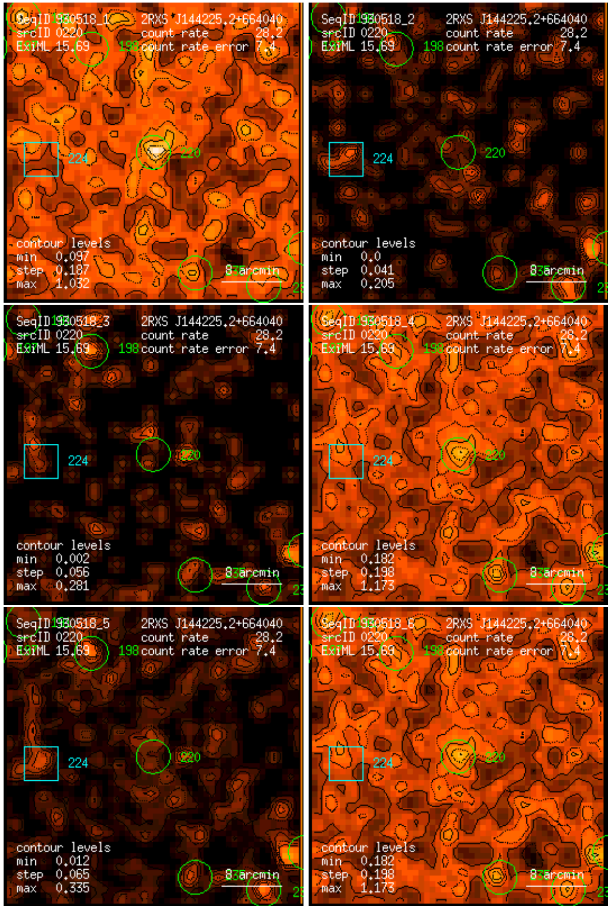
Figure 220: RASS 930518: detection 0220: band rate images, Gaussian filter: (1) PSPC channels 11 – 41, (2) 52 – 90, (3) 91 – 201, (4) 11 – 235, (5) 52 – 201, (6) 11 – 201. Broad band rates in counts/ks. Band rate contour levels in counts/ks/arcmin 2 .
