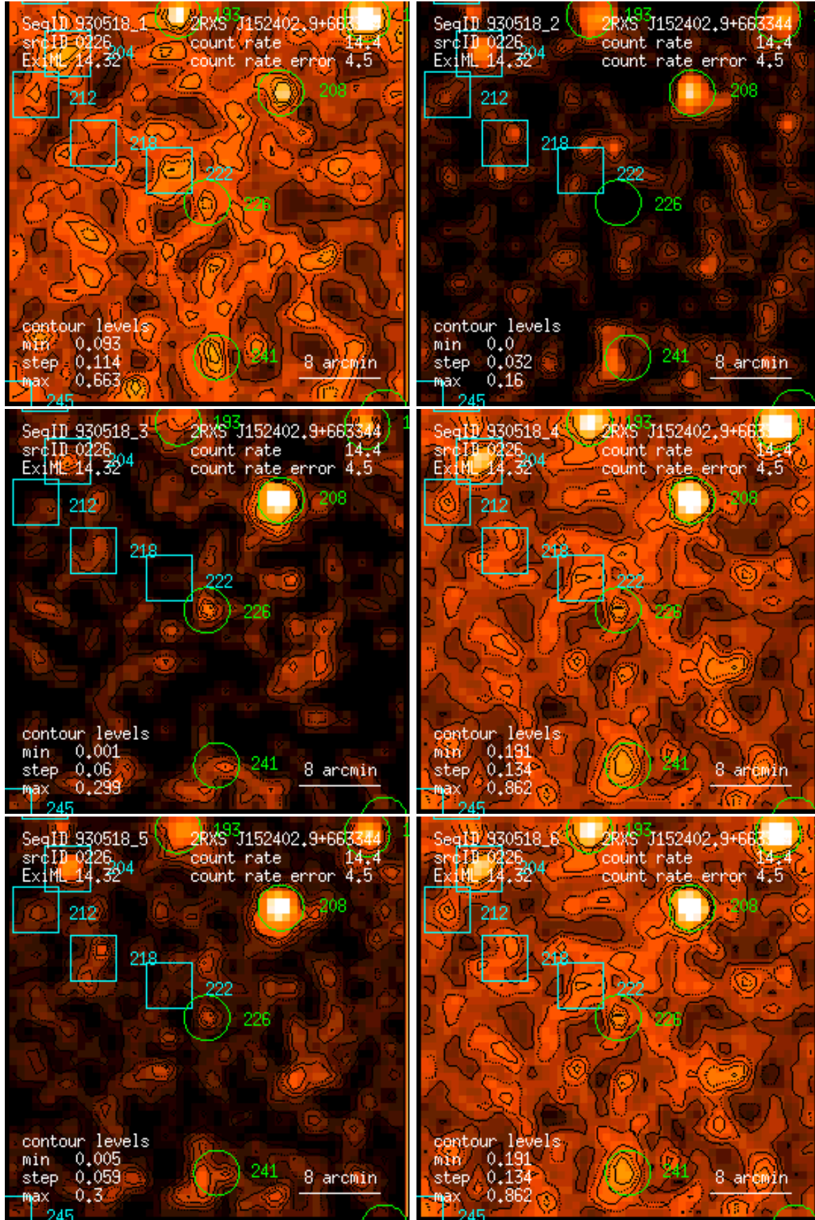
Figure 226: RASS 930518: detection 0226: band rate images, Gaussian filter: (1) PSPC channels 11 – 41, (2) 52 – 90, (3) 91 – 201, (4) 11 – 235, (5) 52 – 201, (6) 11 – 201. Broad band rates in counts/ks. Band rate contour levels in counts/ks/arcmin 2 .
