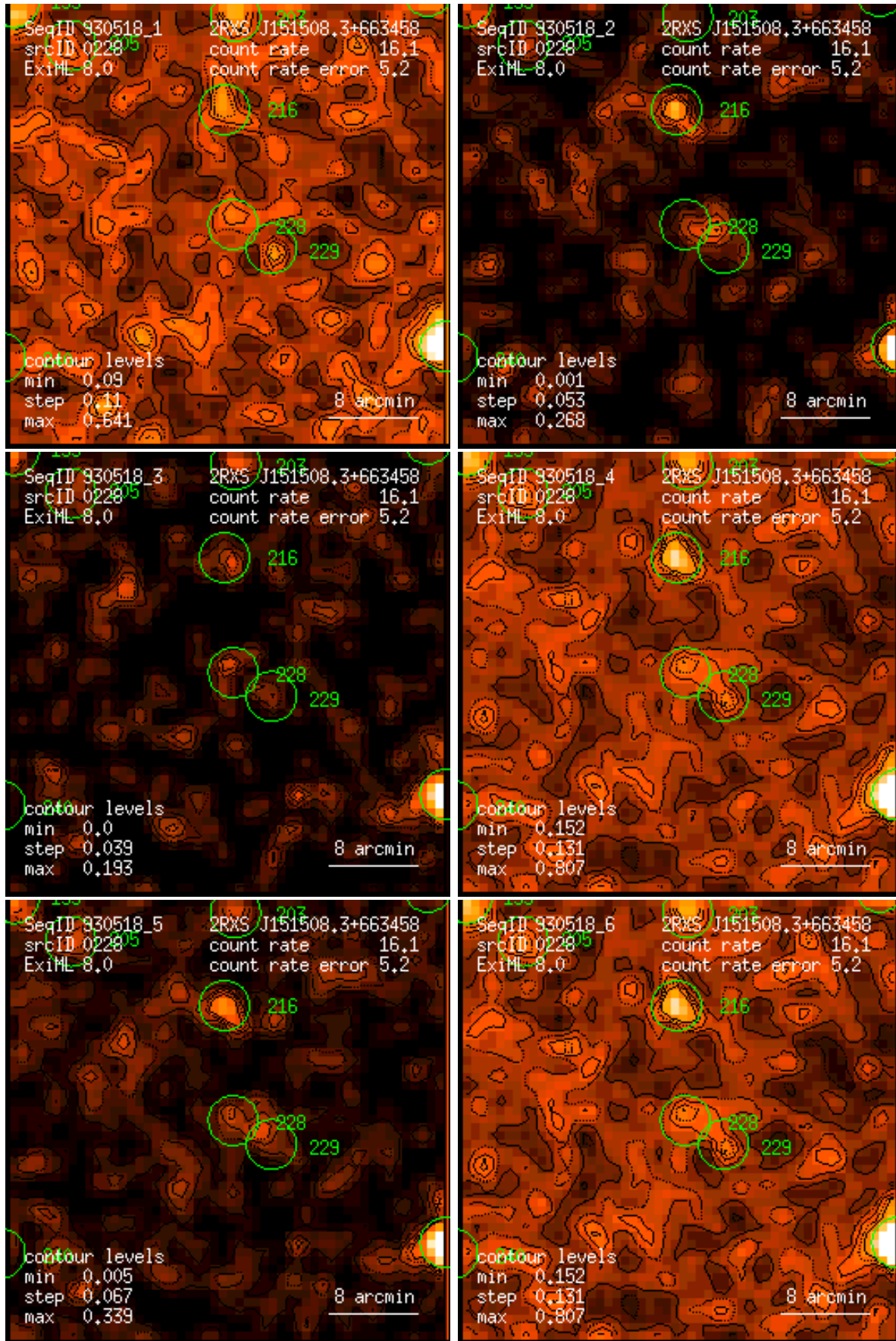
Figure 228: RASS 930518: detection 0228: band rate images, Gaussian filter: (1) PSPC channels 11 – 41, (2) 52 – 90, (3) 91 – 201, (4) 11 – 235, (5) 52 – 201, (6) 11 – 201. Broad band rates in counts/ks. Band rate contour levels in counts/ks/arcmin 2 .
