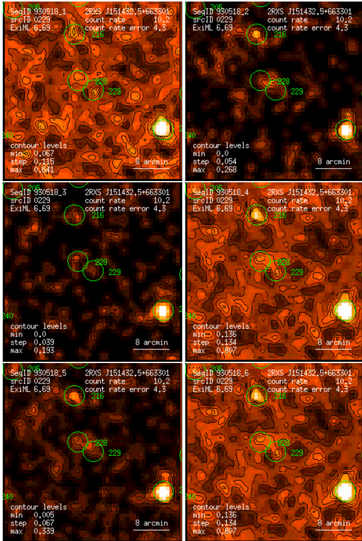
Figure 229: RASS 930518: detection 0229: band rate images, Gaussian filter: (1) PSPC channels 11 – 41, (2) 52 – 90, (3) 91 – 201, (4) 11 – 235, (5) 52 – 201, (6) 11 – 201. Broad band rates in counts/ks. Band rate contour levels in counts/ks/arcmin 2 .
