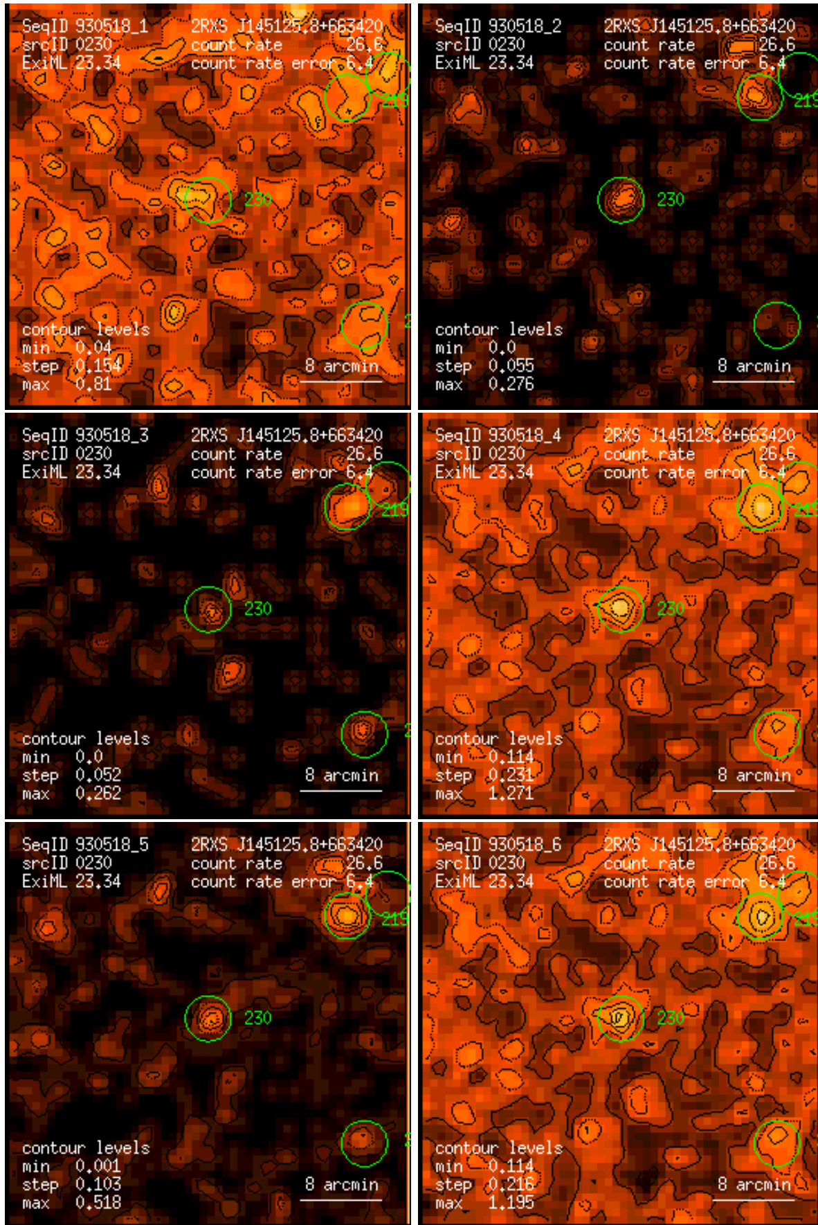
Figure 230: RASS 930518: detection 0230: band rate images, Gaussian filter: (1) PSPC channels 11 – 41, (2) 52 – 90, (3) 91 – 201, (4) 11 – 235, (5) 52 – 201, (6) 11 – 201. Broad band rates in counts/ks. Band rate contour levels in counts/ks/arcmin 2 .
