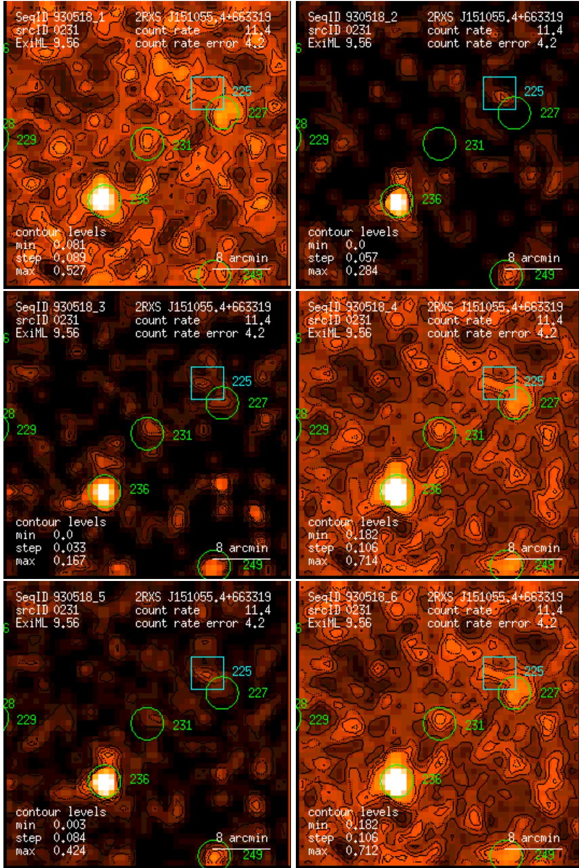
Figure 231: RASS 930518: detection 0231: band rate images, Gaussian filter: (1) PSPC channels 11 – 41, (2) 52 – 90, (3) 91 – 201, (4) 11 – 235, (5) 52 – 201, (6) 11 – 201. Broad band rates in counts/ks. Band rate contour levels in counts/ks/arcmin 2 .
