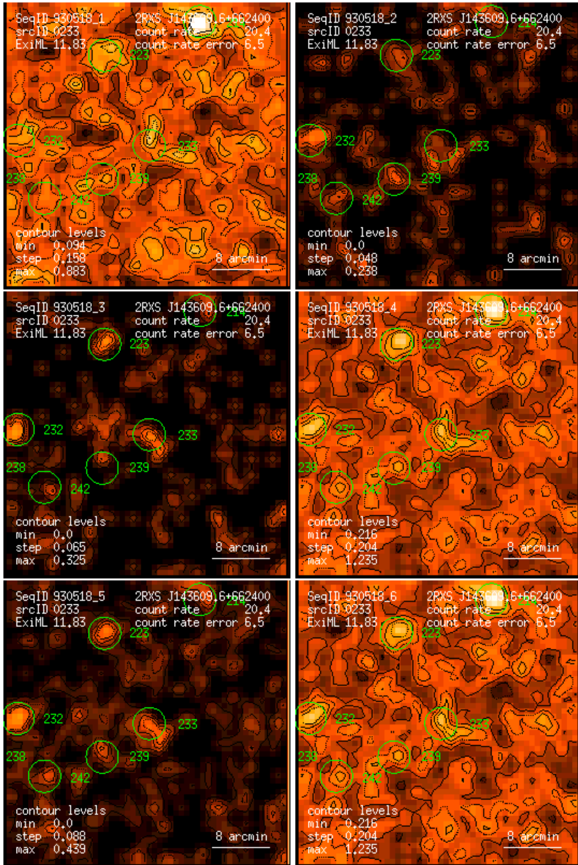
Figure 233: RASS 930518: detection 0233: band rate images, Gaussian filter: (1) PSPC channels 11 – 41, (2) 52 – 90, (3) 91 – 201, (4) 11 – 235, (5) 52 – 201, (6) 11 – 201. Broad band rates in counts/ks. Band rate contour levels in counts/ks/arcmin 2 .
