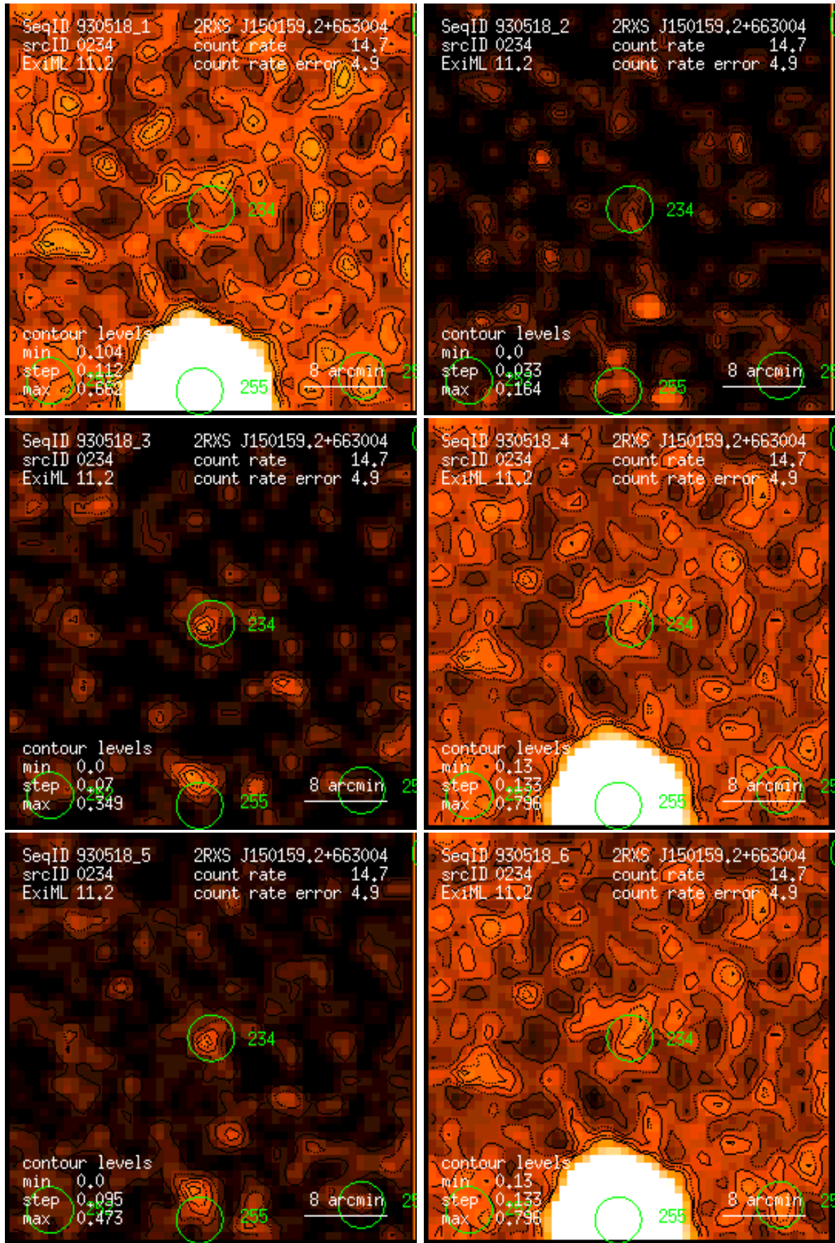
Figure 234: RASS 930518: detection 0234: band rate images, Gaussian filter: (1) PSPC channels 11 – 41, (2) 52 – 90, (3) 91 – 201, (4) 11 – 235, (5) 52 – 201, (6) 11 – 201. Broad band rates in counts/ks. Band rate contour levels in counts/ks/arcmin 2 .
