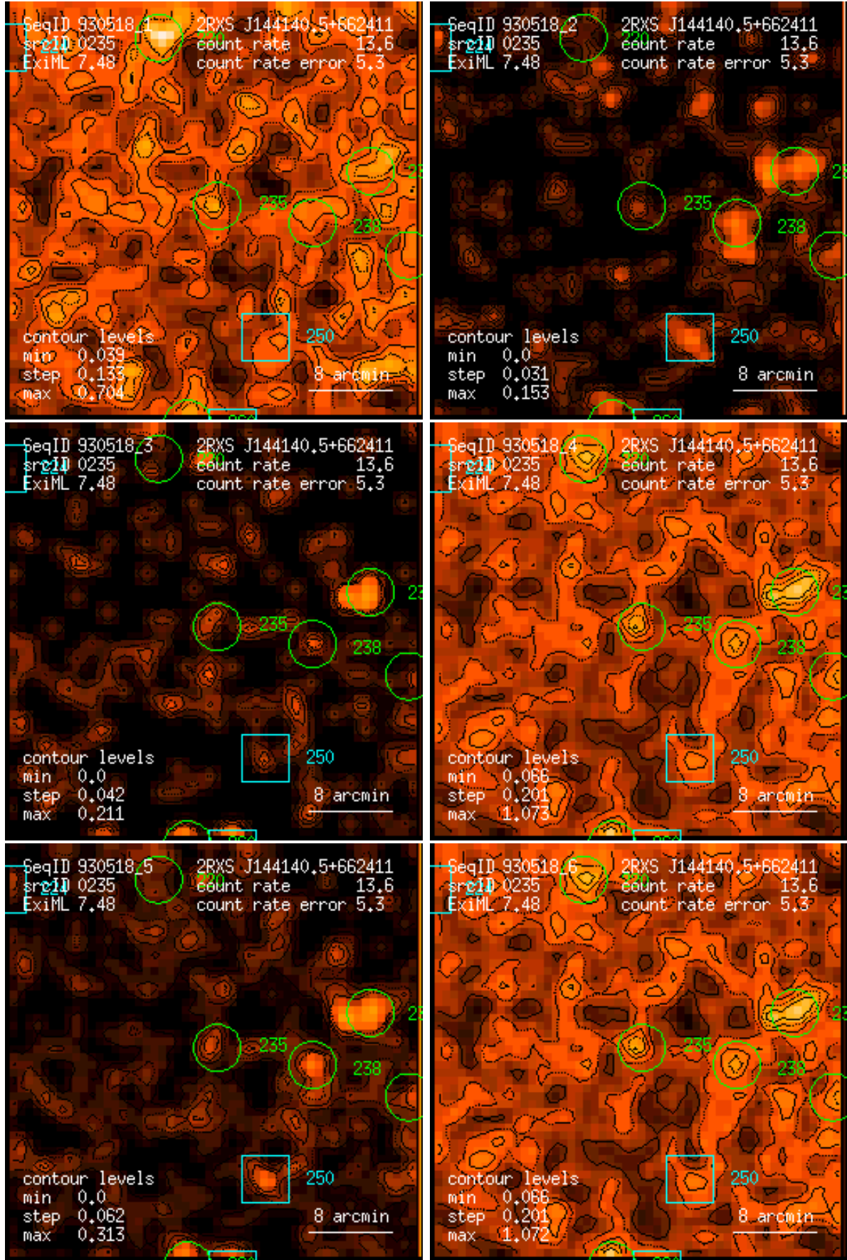
Figure 235: RASS 930518: detection 0235: band rate images, Gaussian filter: (1) PSPC channels 11 – 41, (2) 52 – 90, (3) 91 – 201, (4) 11 – 235, (5) 52 – 201, (6) 11 – 201. Broad band rates in counts/ks. Band rate contour levels in counts/ks/arcmin 2 .
