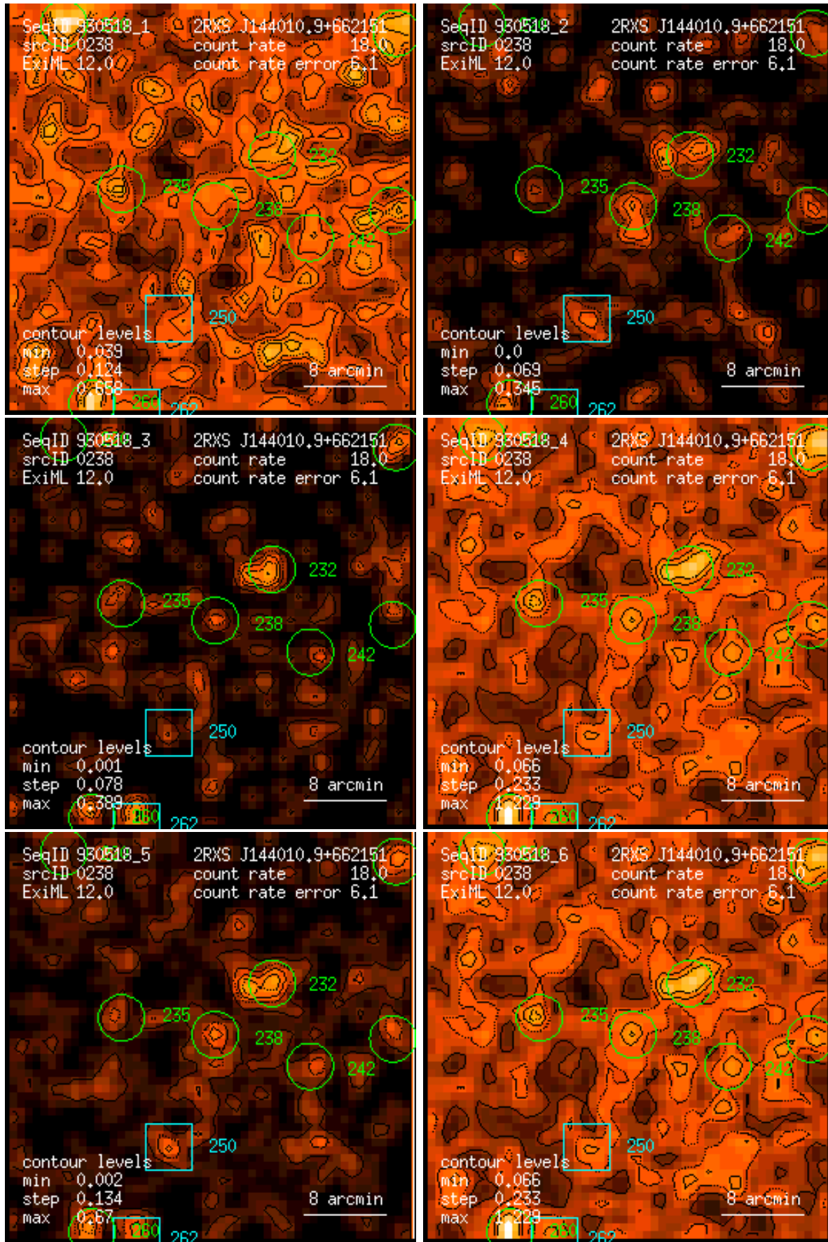
Figure 238: RASS 930518: detection 0238: band rate images, Gaussian filter: (1) PSPC channels 11 – 41, (2) 52 – 90, (3) 91 – 201, (4) 11 – 235, (5) 52 – 201, (6) 11 – 201. Broad band rates in counts/ks. Band rate contour levels in counts/ks/arcmin 2 .
