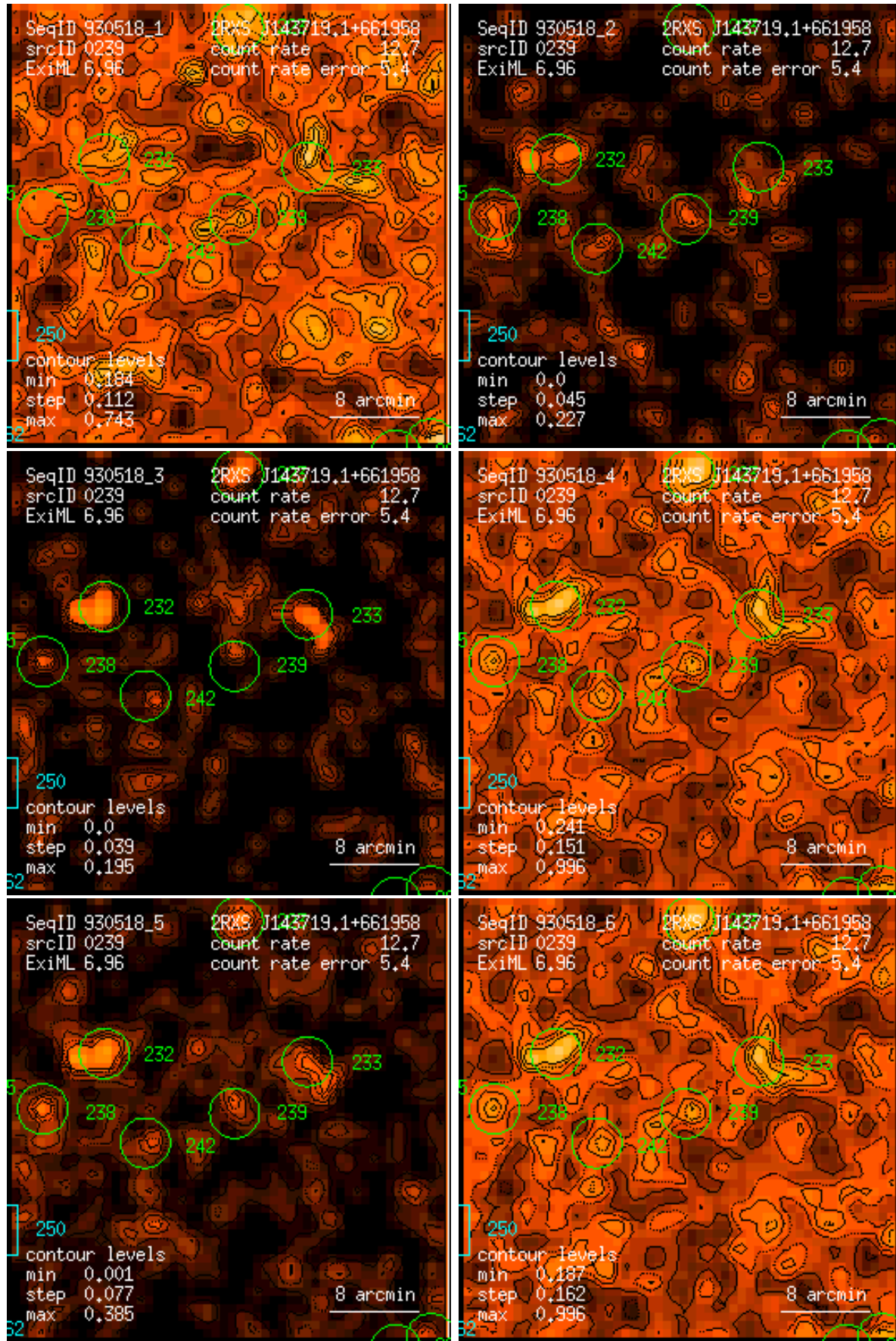
Figure 239: RASS 930518: detection 0239: band rate images, Gaussian filter: (1) PSPC channels 11 – 41, (2) 52 – 90, (3) 91 – 201, (4) 11 – 235, (5) 52 – 201, (6) 11 – 201. Broad band rates in counts/ks. Band rate contour levels in counts/ks/arcmin 2 .
