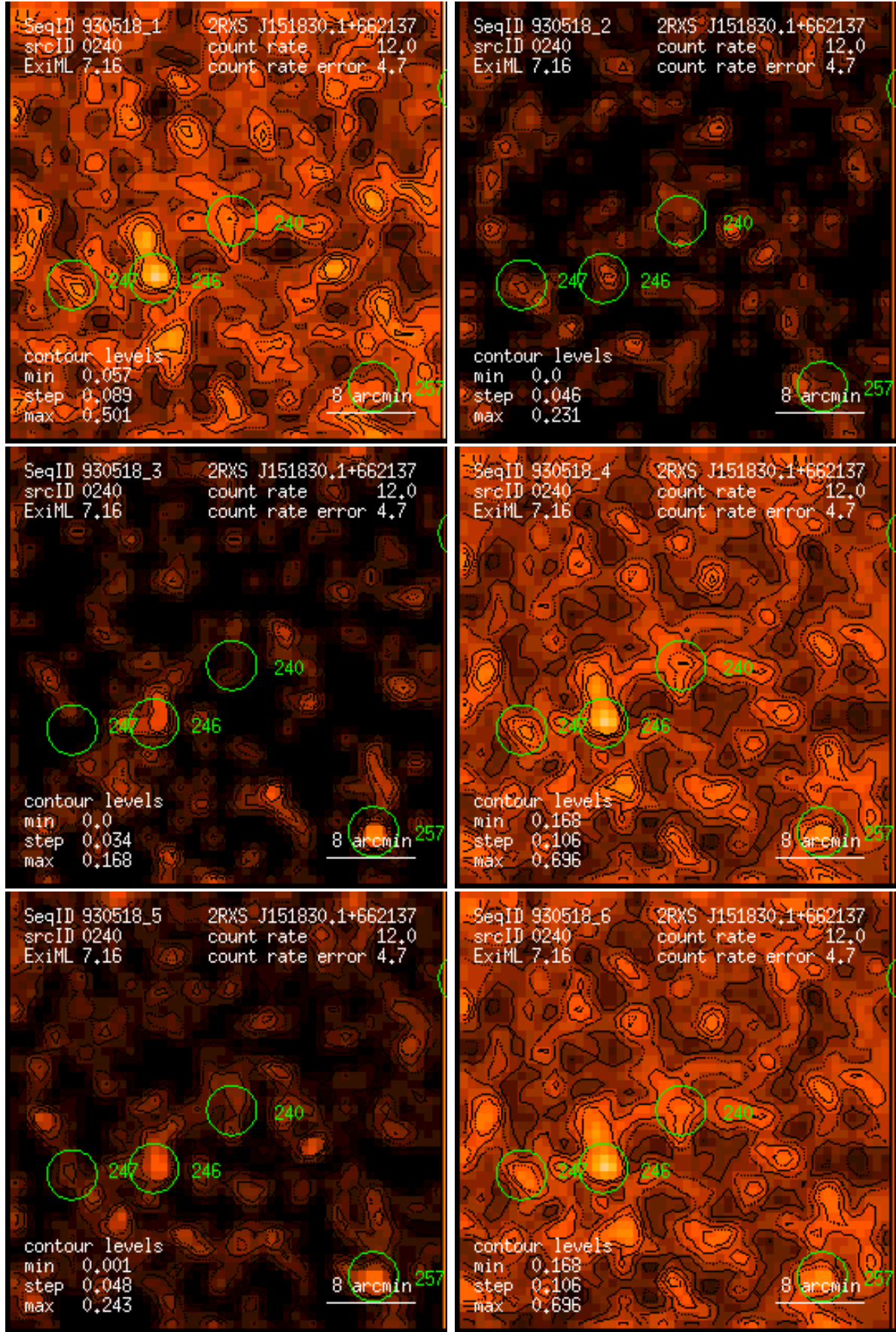
Figure 240: RASS 930518: detection 0240: band rate images, Gaussian filter: (1) PSPC channels 11 – 41, (2) 52 – 90, (3) 91 – 201, (4) 11 – 235, (5) 52 – 201, (6) 11 – 201. Broad band rates in counts/ks. Band rate contour levels in counts/ks/arcmin 2 .
