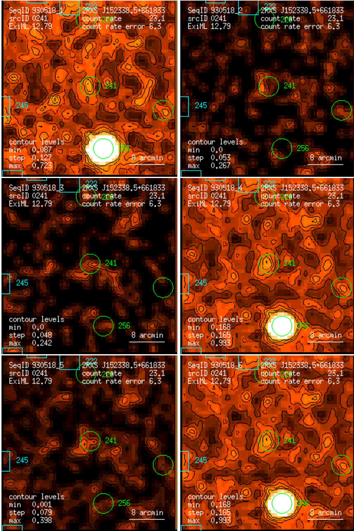
Figure 241: RASS 930518: detection 0241: band rate images, Gaussian filter: (1) PSPC channels 11 – 41, (2) 52 – 90, (3) 91 – 201, (4) 11 – 235, (5) 52 – 201, (6) 11 – 201. Broad band rates in counts/ks. Band rate contour levels in counts/ks/arcmin 2 .
