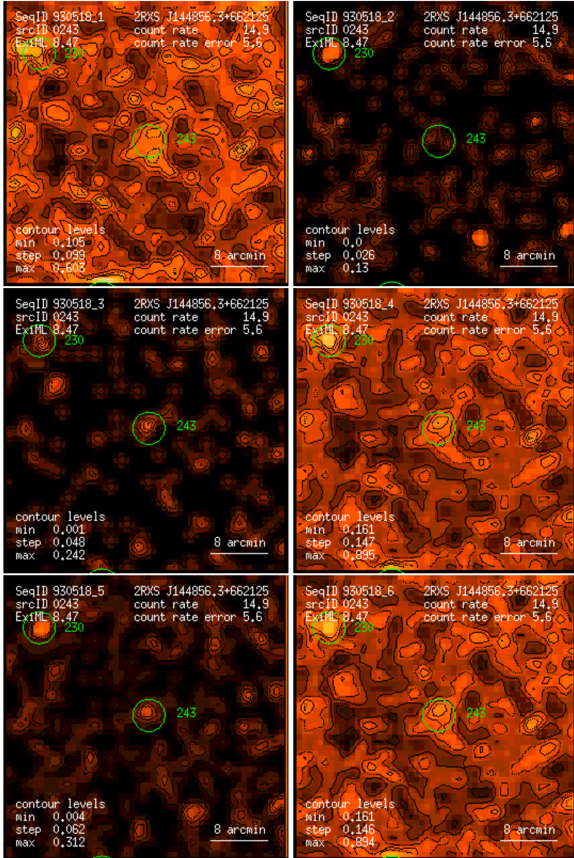
Figure 243: RASS 930518: detection 0243: band rate images, Gaussian filter: (1) PSPC channels 11 – 41, (2) 52 – 90, (3) 91 – 201, (4) 11 – 235, (5) 52 – 201, (6) 11 – 201. Broad band rates in counts/ks. Band rate contour levels in counts/ks/arcmin 2 .
