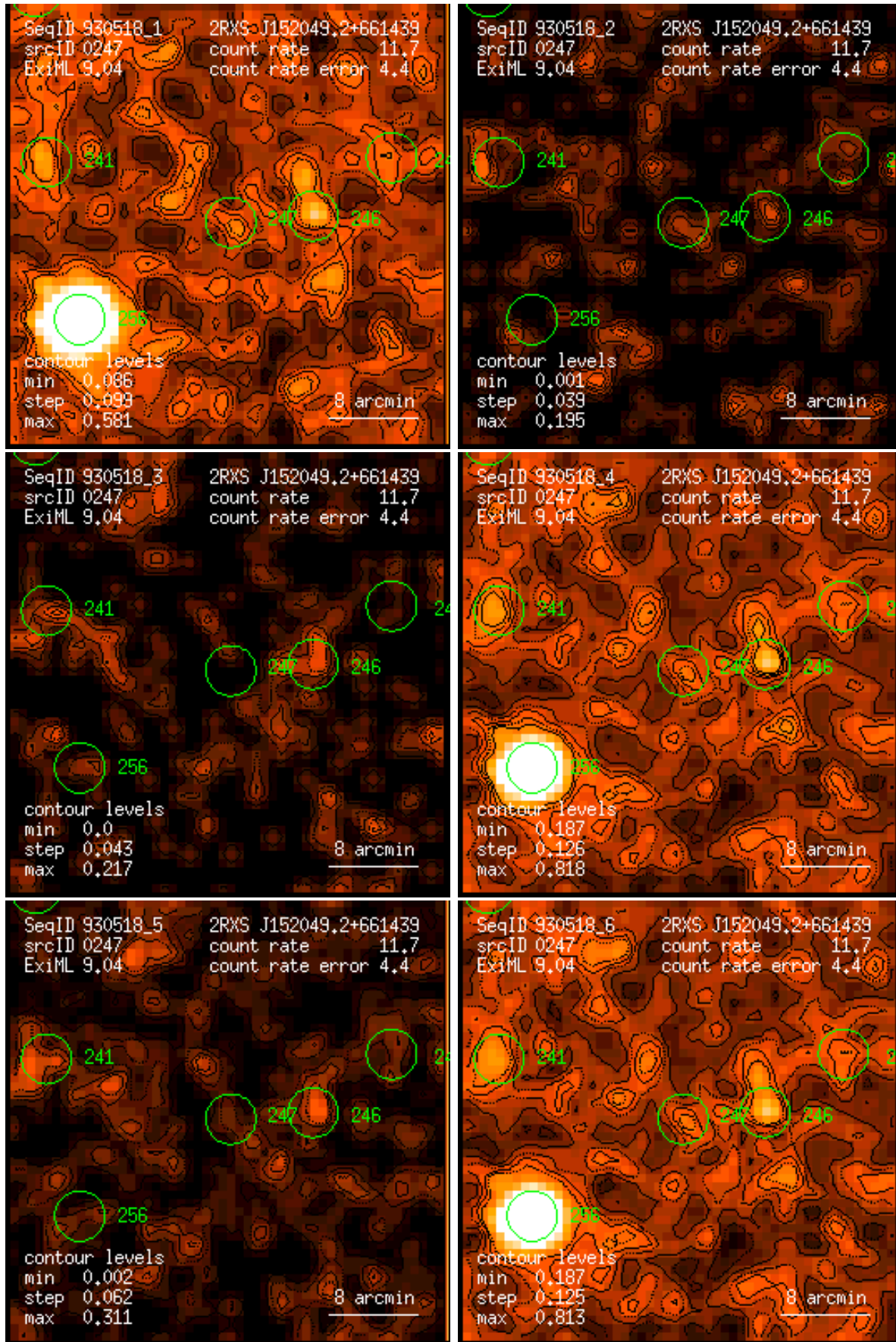
Figure 247: RASS 930518: detection 0247: band rate images, Gaussian filter: (1) PSPC channels 11 – 41, (2) 52 – 90, (3) 91 – 201, (4) 11 – 235, (5) 52 – 201, (6) 11 – 201. Broad band rates in counts/ks. Band rate contour levels in counts/ks/arcmin 2 .
