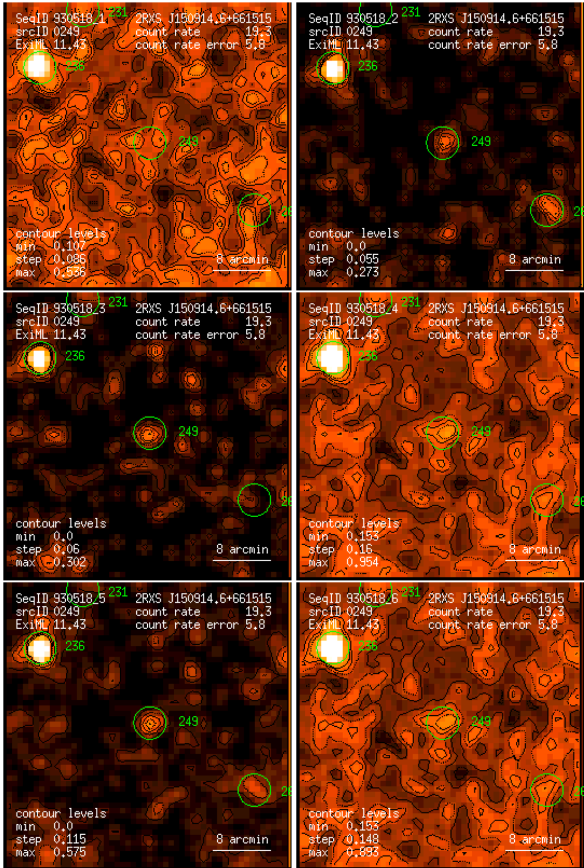
Figure 249: RASS 930518: detection 0249: band rate images, Gaussian filter: (1) PSPC channels 11 – 41, (2) 52 – 90, (3) 91 – 201, (4) 11 – 235, (5) 52 – 201, (6) 11 – 201. Broad band rates in counts/ks. Band rate contour levels in counts/ks/arcmin 2 .
