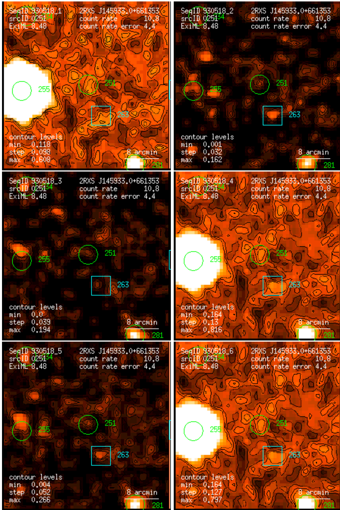
Figure 251: RASS 930518: detection 0251: band rate images, Gaussian filter: (1) PSPC channels 11 – 41, (2) 52 – 90, (3) 91 – 201, (4) 11 – 235, (5) 52 – 201, (6) 11 – 201. Broad band rates in counts/ks. Band rate contour levels in counts/ks/arcmin 2 .
