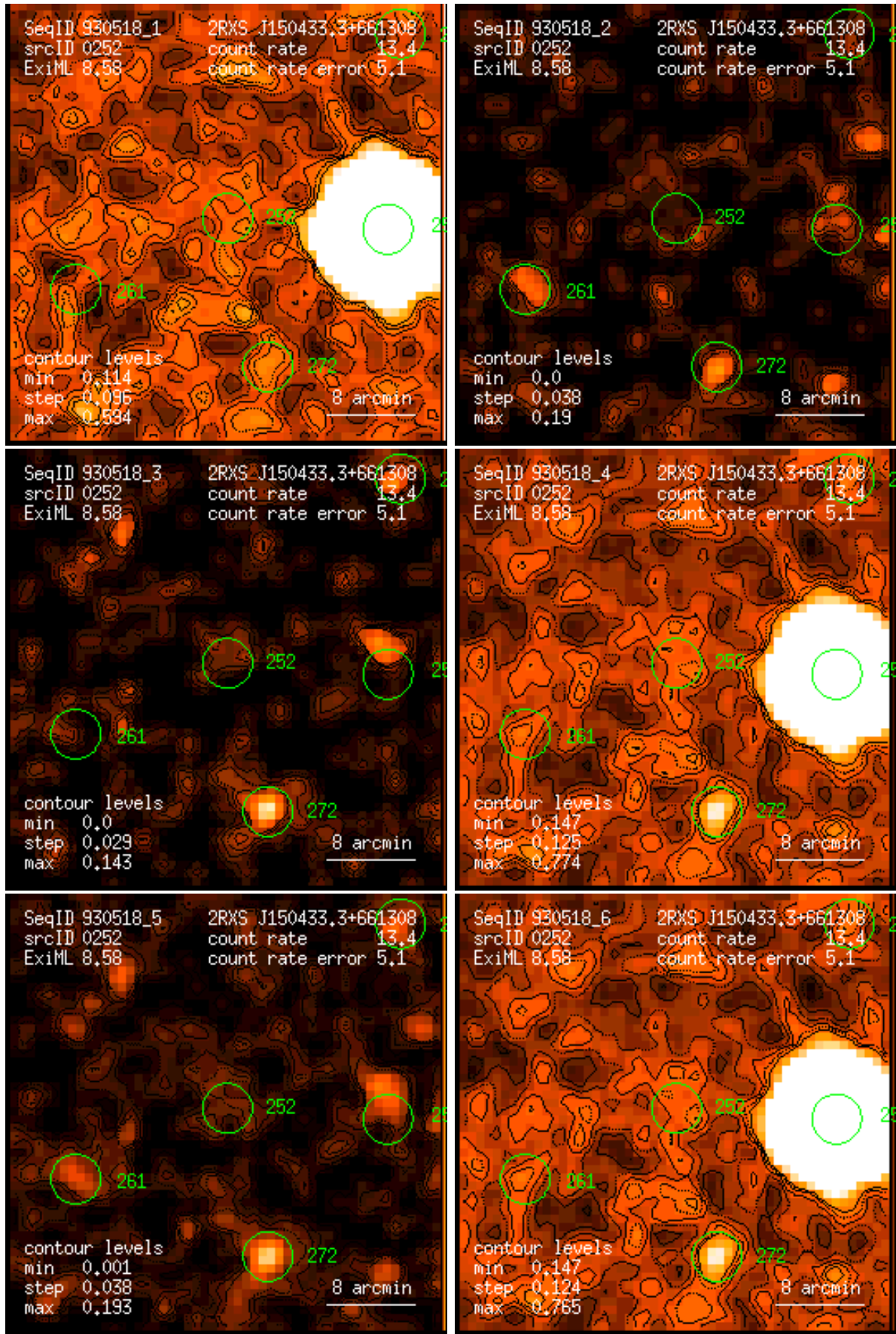
Figure 252: RASS 930518: detection 0252: band rate images, Gaussian filter: (1) PSPC channels 11 – 41, (2) 52 – 90, (3) 91 – 201, (4) 11 – 235, (5) 52 – 201, (6) 11 – 201. Broad band rates in counts/ks. Band rate contour levels in counts/ks/arcmin 2 .
