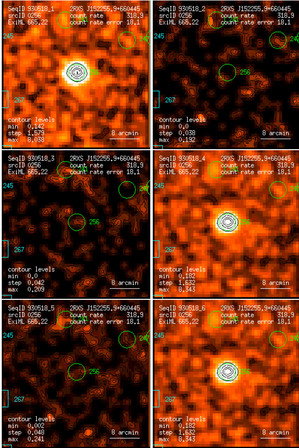
Figure 256: RASS 930518: detection 0256: band rate images, Gaussian filter: (1) PSPC channels 11 – 41, (2) 52 – 90, (3) 91 – 201, (4) 11 – 235, (5) 52 – 201, (6) 11 – 201. Broad band rates in counts/ks. Band rate contour levels in counts/ks/arcmin 2 .
