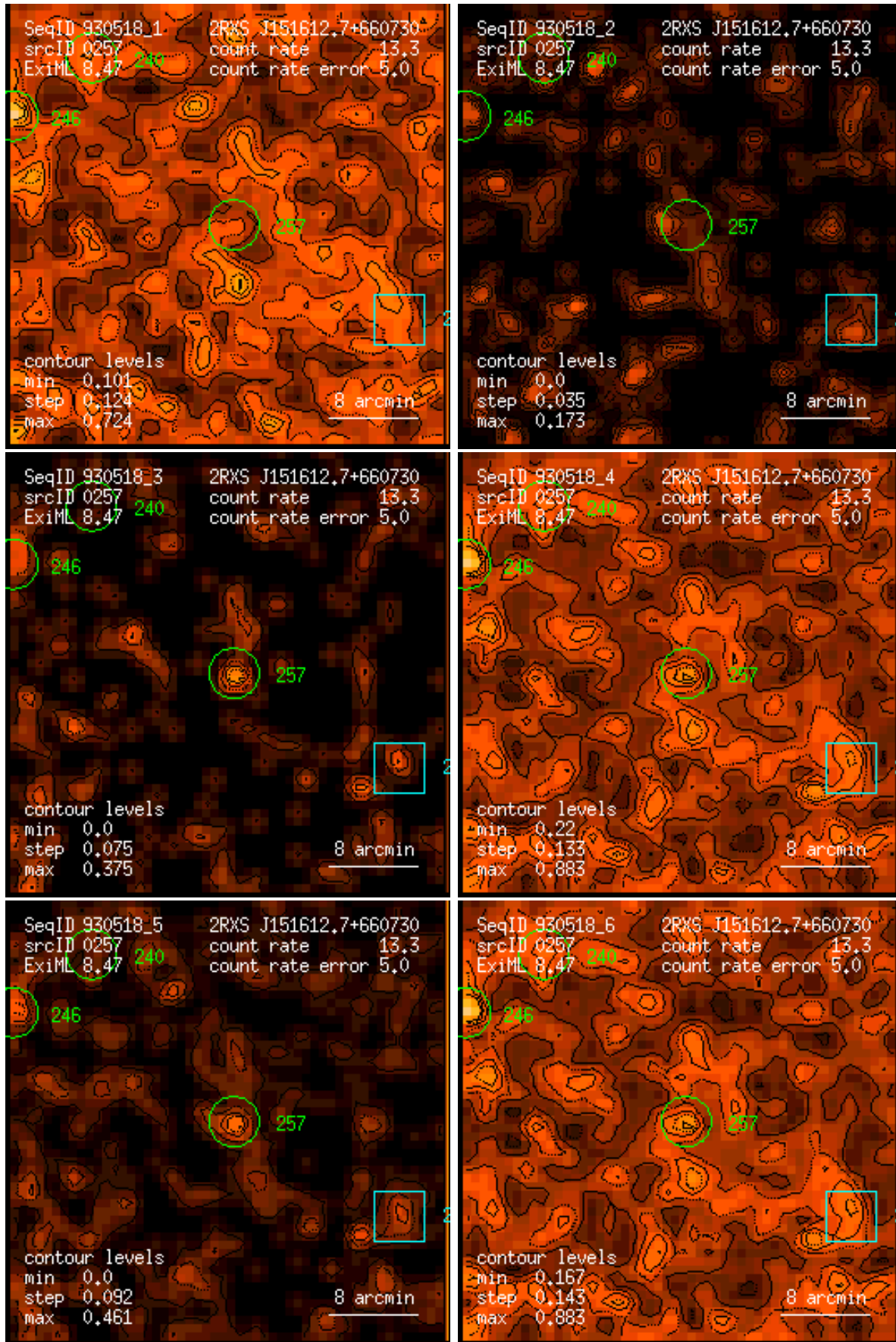
Figure 257: RASS 930518: detection 0257: band rate images, Gaussian filter: (1) PSPC channels 11 – 41, (2) 52 – 90, (3) 91 – 201, (4) 11 – 235, (5) 52 – 201, (6) 11 – 201. Broad band rates in counts/ks. Band rate contour levels in counts/ks/arcmin 2 .
