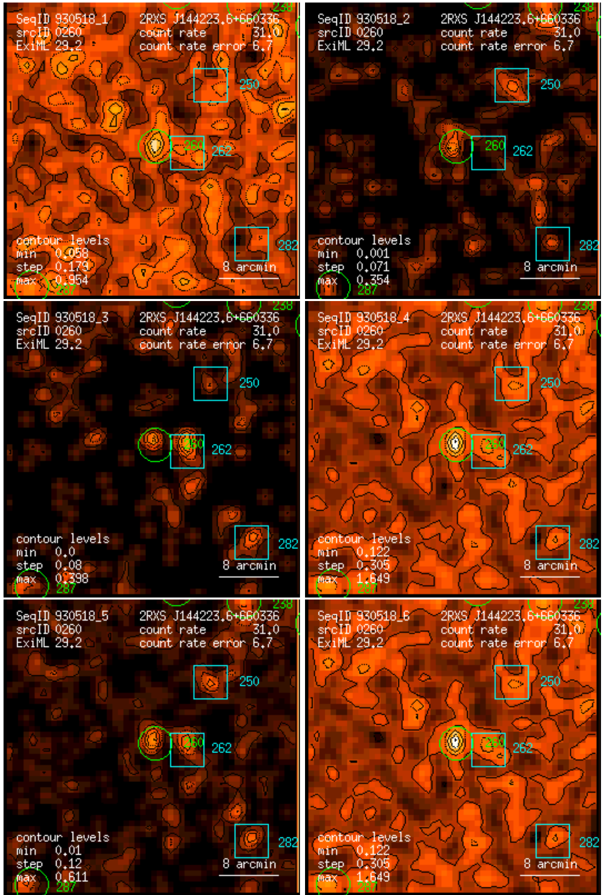
Figure 260: RASS 930518: detection 0260: band rate images, Gaussian filter: (1) PSPC channels 11 – 41, (2) 52 – 90, (3) 91 – 201, (4) 11 – 235, (5) 52 – 201, (6) 11 – 201. Broad band rates in counts/ks. Band rate contour levels in counts/ks/arcmin 2 .
