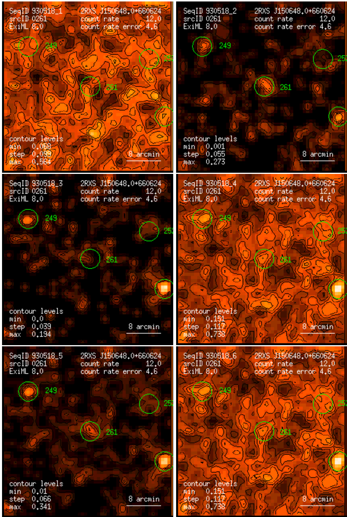
Figure 261: RASS 930518: detection 0261: band rate images, Gaussian filter: (1) PSPC channels 11 – 41, (2) 52 – 90, (3) 91 – 201, (4) 11 – 235, (5) 52 – 201, (6) 11 – 201. Broad band rates in counts/ks. Band rate contour levels in counts/ks/arcmin 2 .
