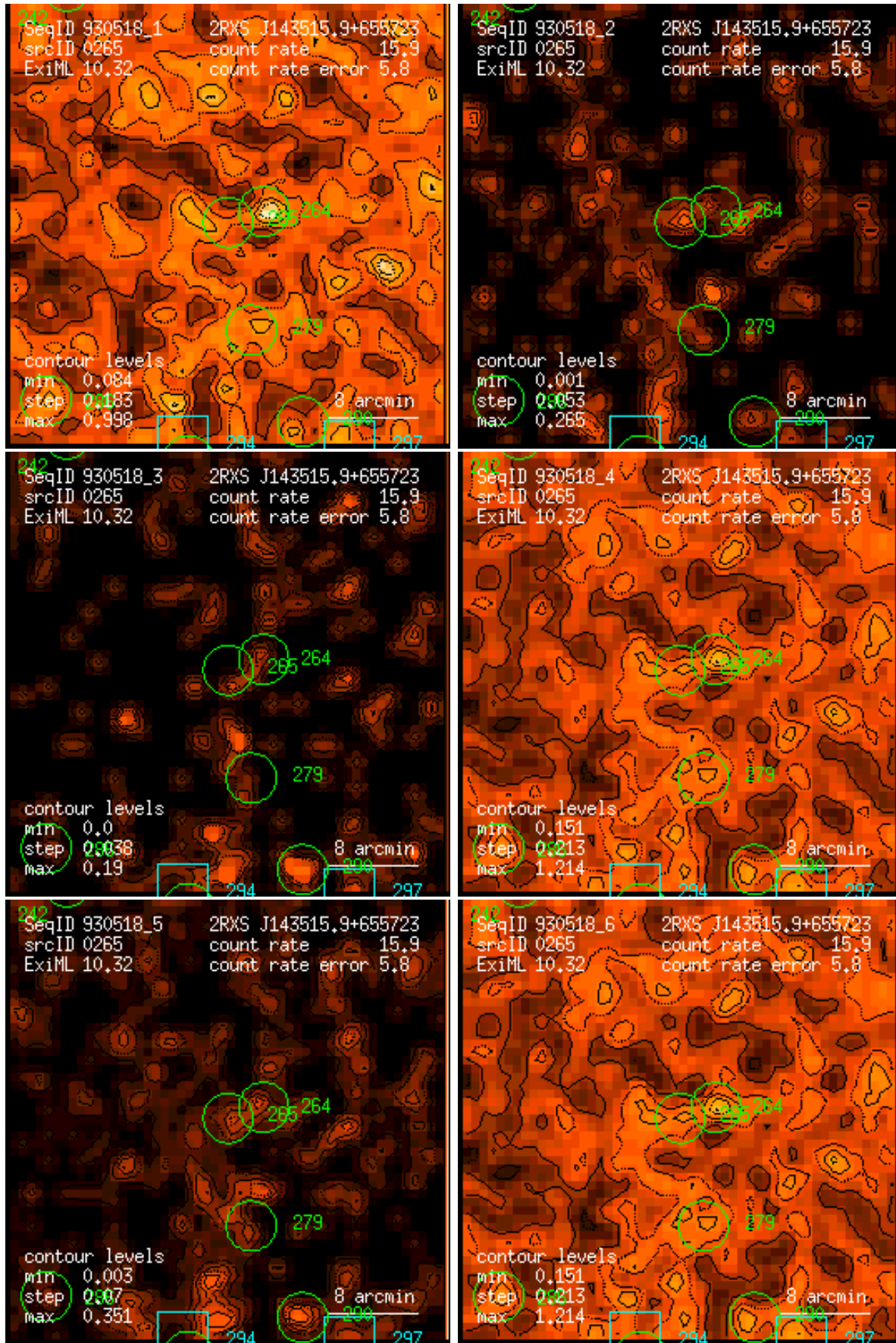
Figure 265: RASS 930518: detection 0265: band rate images, Gaussian filter: (1) PSPC channels 11 – 41, (2) 52 – 90, (3) 91 – 201, (4) 11 – 235, (5) 52 – 201, (6) 11 – 201. Broad band rates in counts/ks. Band rate contour levels in counts/ks/arcmin 2 .
