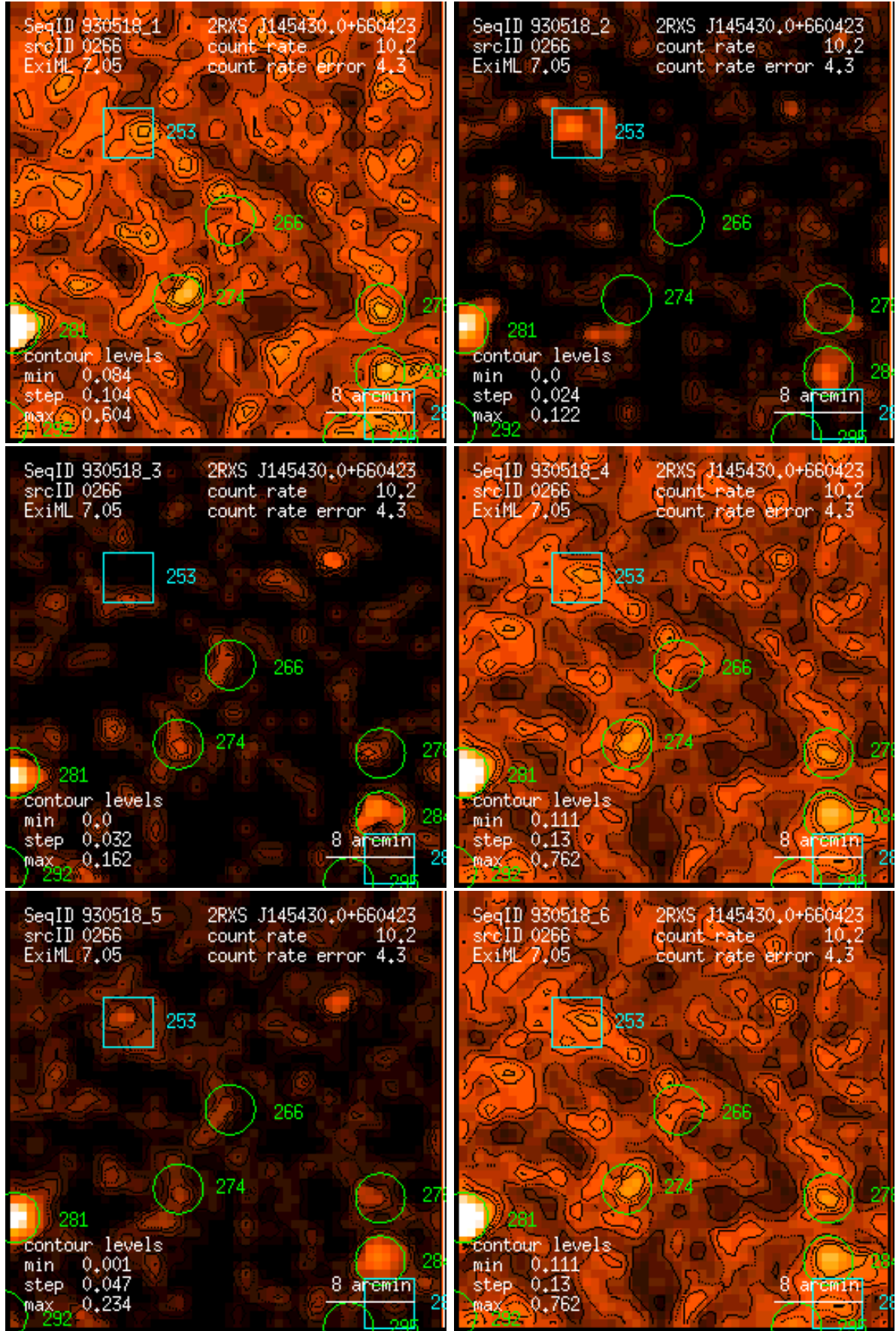
Figure 266: RASS 930518: detection 0266: band rate images, Gaussian filter: (1) PSPC channels 11 – 41, (2) 52 – 90, (3) 91 – 201, (4) 11 – 235, (5) 52 – 201, (6) 11 – 201. Broad band rates in counts/ks. Band rate contour levels in counts/ks/arcmin 2 .
