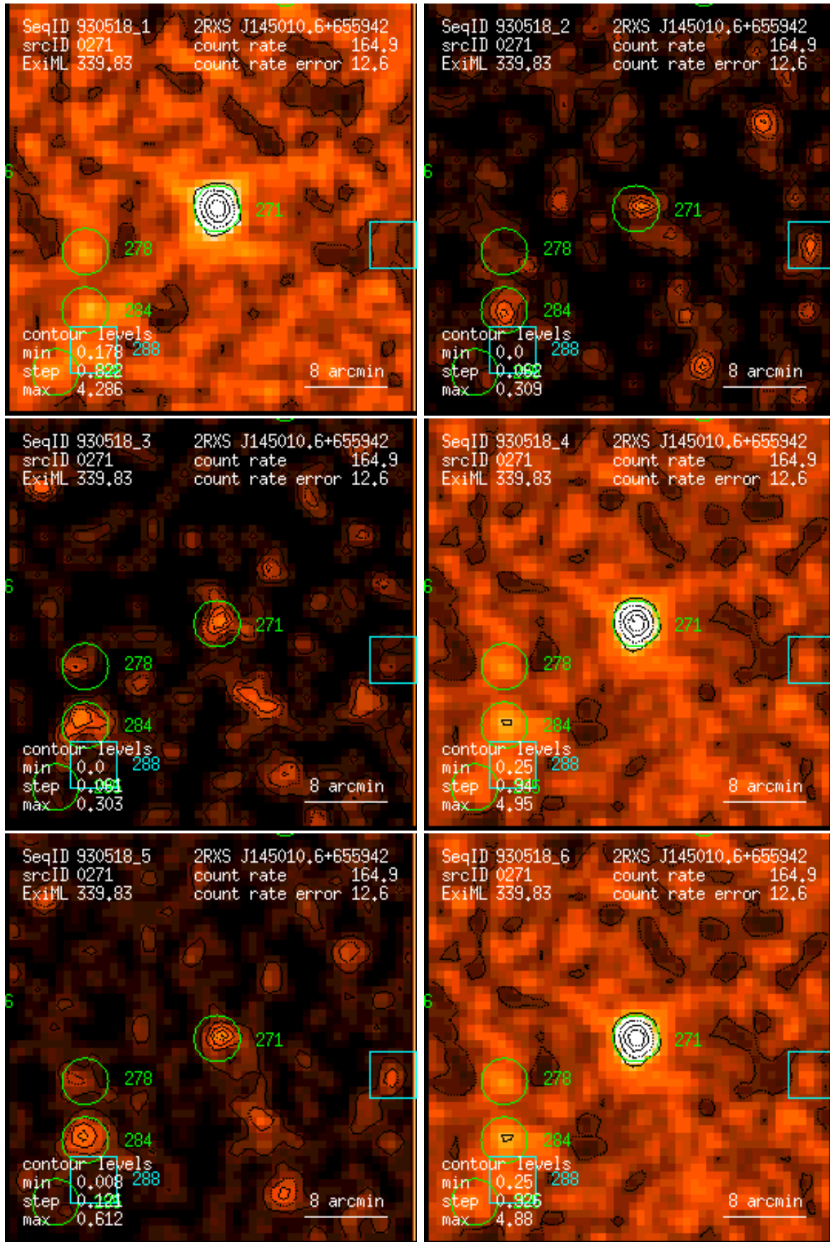
Figure 271: RASS 930518: detection 0271: band rate images, Gaussian filter: (1) PSPC channels 11 – 41, (2) 52 – 90, (3) 91 – 201, (4) 11 – 235, (5) 52 – 201, (6) 11 – 201. Broad band rates in counts/ks. Band rate contour levels in counts/ks/arcmin 2 .
