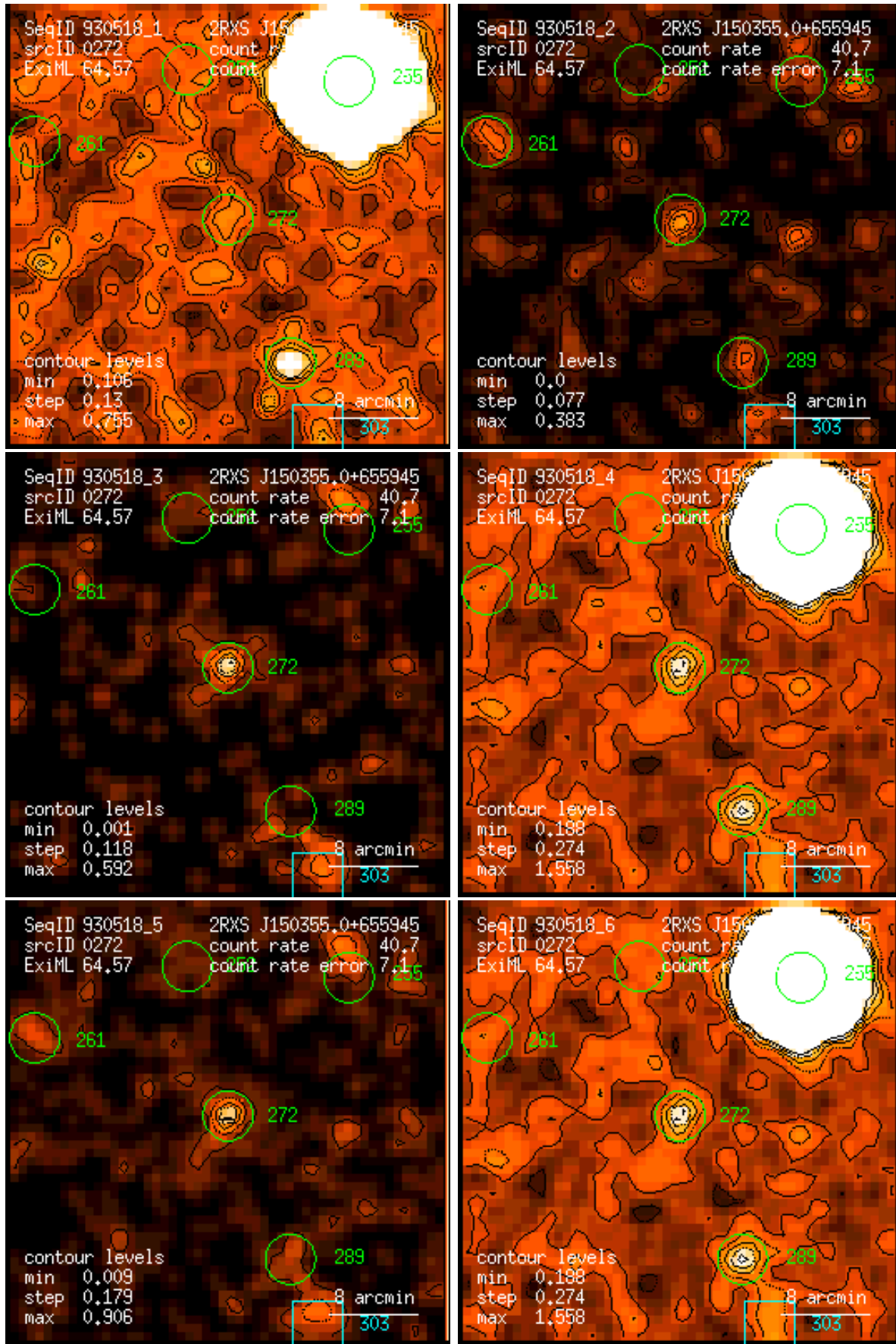
Figure 272: RASS 930518: detection 0272: band rate images, Gaussian filter: (1) PSPC channels 11 – 41, (2) 52 – 90, (3) 91 – 201, (4) 11 – 235, (5) 52 – 201, (6) 11 – 201. Broad band rates in counts/ks. Band rate contour levels in counts/ks/arcmin 2 .
