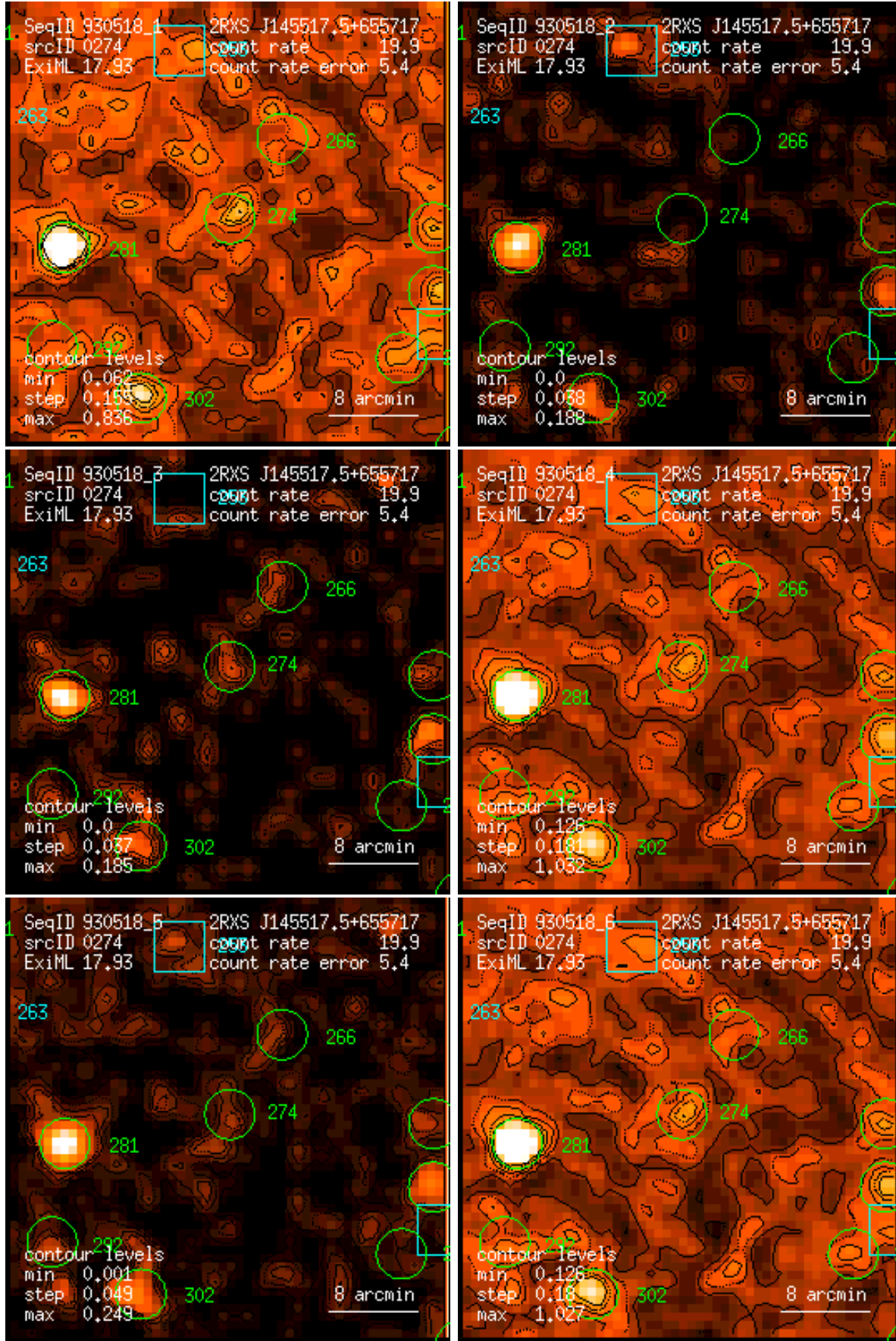
Figure 274: RASS 930518: detection 0274: band rate images, Gaussian filter: (1) PSPC channels 11 – 41, (2) 52 – 90, (3) 91 – 201, (4) 11 – 235, (5) 52 – 201, (6) 11 – 201. Broad band rates in counts/ks. Band rate contour levels in counts/ks/arcmin 2 .
