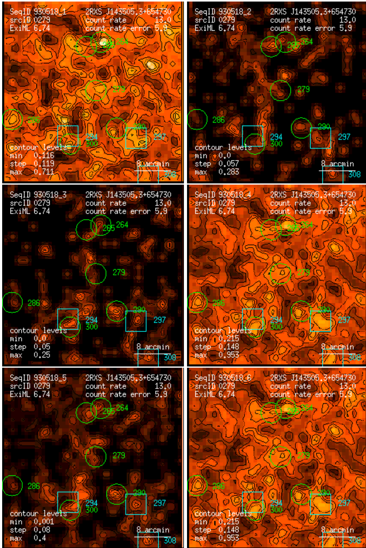
Figure 279: RASS 930518: detection 0279: band rate images, Gaussian filter: (1) PSPC channels 11 – 41, (2) 52 – 90, (3) 91 – 201, (4) 11 – 235, (5) 52 – 201, (6) 11 – 201. Broad band rates in counts/ks. Band rate contour levels in counts/ks/arcmin 2 .
