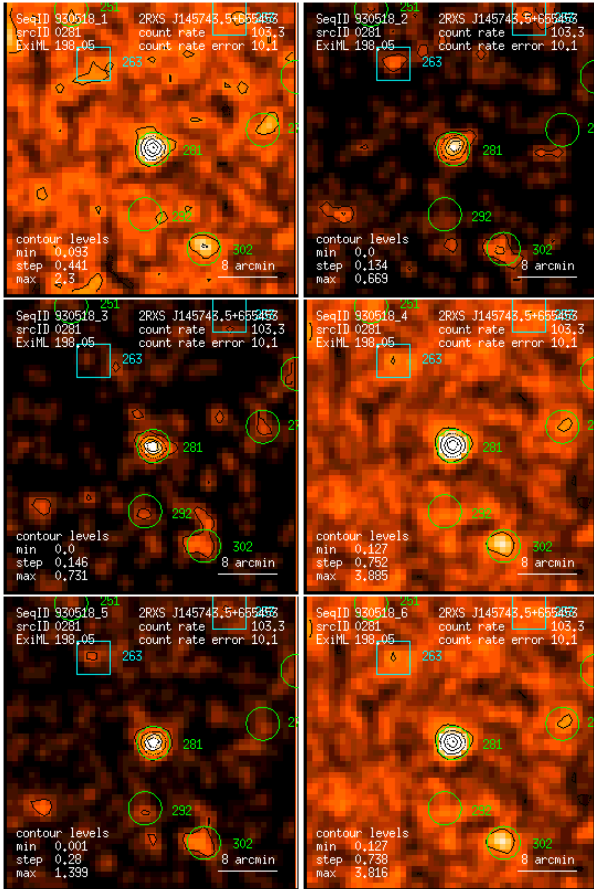
Figure 281: RASS 930518: detection 0281: band rate images, Gaussian filter: (1) PSPC channels 11 – 41, (2) 52 – 90, (3) 91 – 201, (4) 11 – 235, (5) 52 – 201, (6) 11 – 201. Broad band rates in counts/ks. Band rate contour levels in counts/ks/arcmin 2 .
