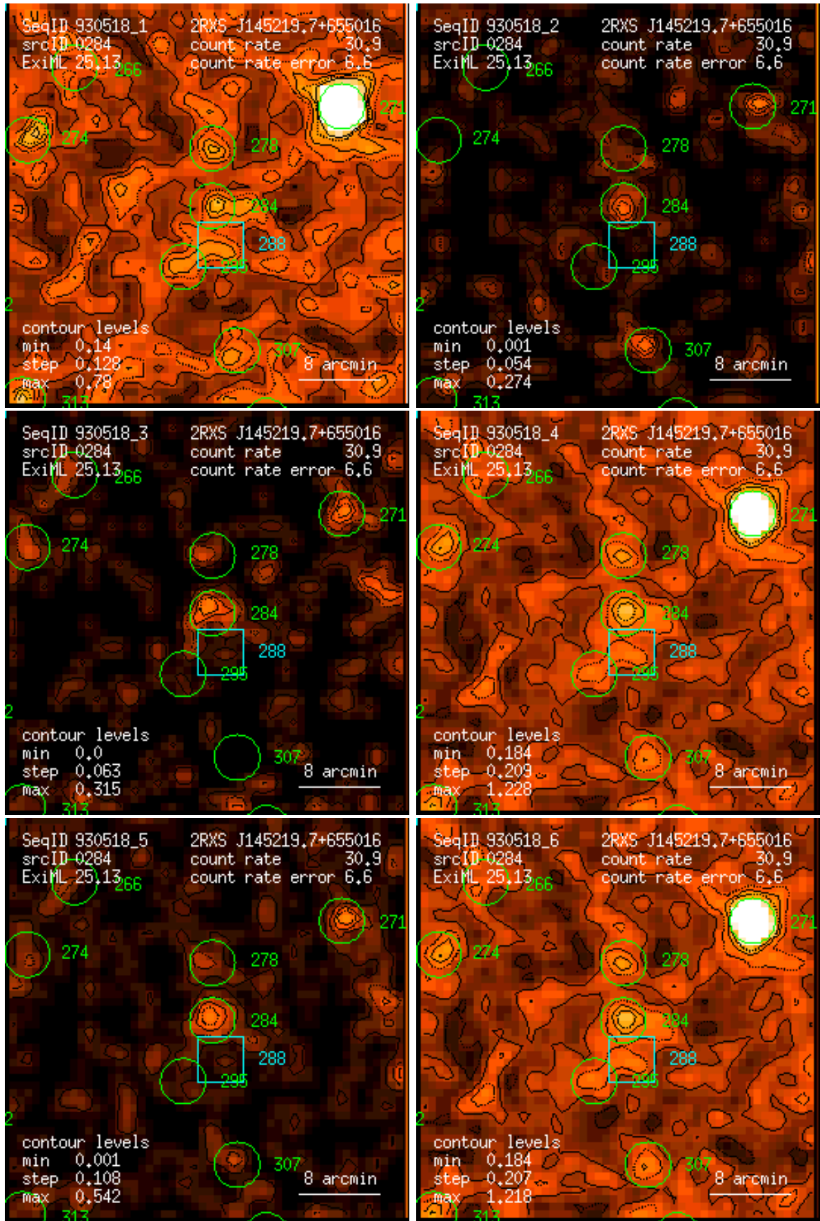
Figure 284: RASS 930518: detection 0284: band rate images, Gaussian filter: (1) PSPC channels 11 – 41, (2) 52 – 90, (3) 91 – 201, (4) 11 – 235, (5) 52 – 201, (6) 11 – 201. Broad band rates in counts/ks. Band rate contour levels in counts/ks/arcmin 2 .
