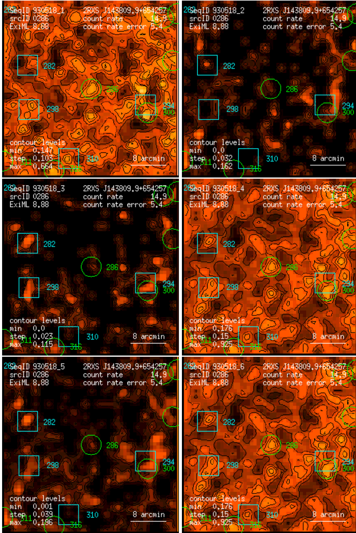
Figure 286: RASS 930518: detection 0286: band rate images, Gaussian filter: (1) PSPC channels 11 – 41, (2) 52 – 90, (3) 91 – 201, (4) 11 – 235, (5) 52 – 201, (6) 11 – 201. Broad band rates in counts/ks. Band rate contour levels in counts/ks/arcmin 2 .
