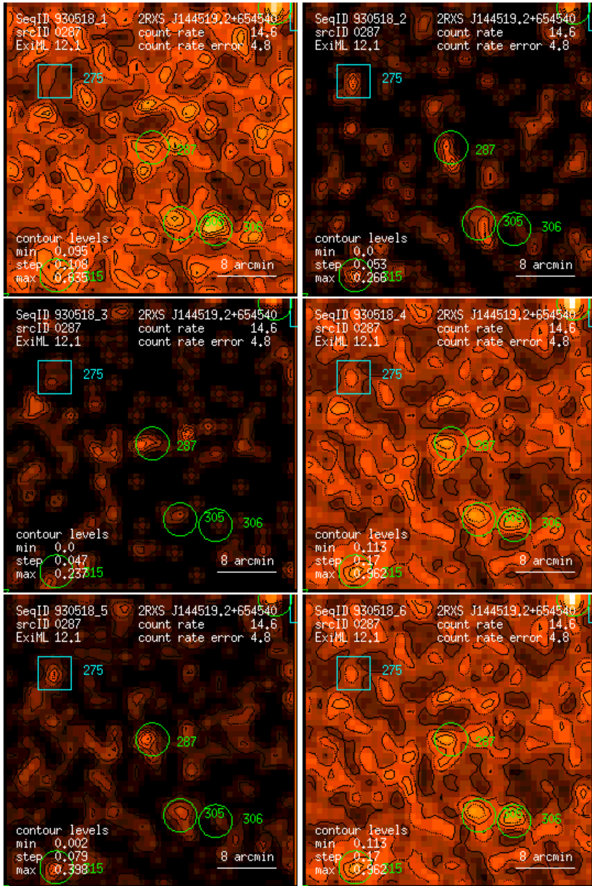
Figure 287: RASS 930518: detection 0287: band rate images, Gaussian filter: (1) PSPC channels 11 – 41, (2) 52 – 90, (3) 91 – 201, (4) 11 – 235, (5) 52 – 201, (6) 11 – 201. Broad band rates in counts/ks. Band rate contour levels in counts/ks/arcmin 2 .
