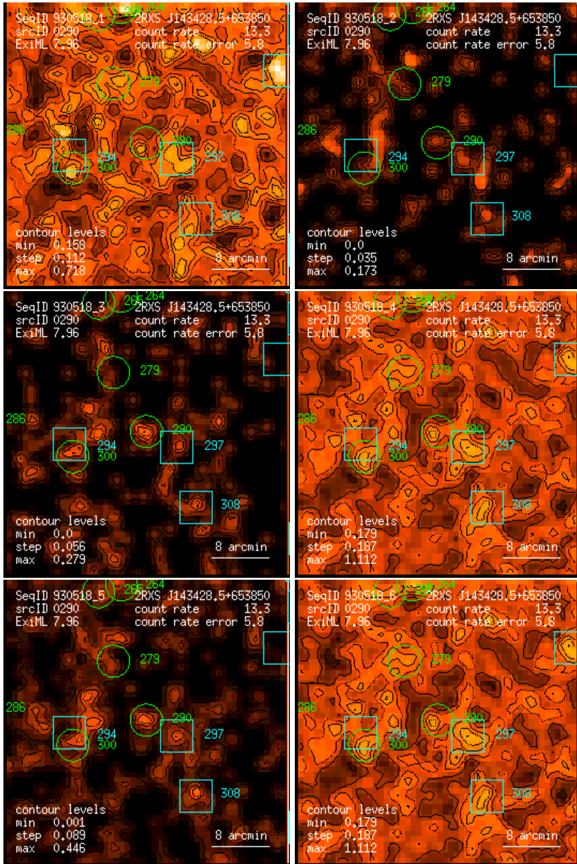
Figure 290: RASS 930518: detection 0290: band rate images, Gaussian filter: (1) PSPC channels 11 – 41, (2) 52 – 90, (3) 91 – 201, (4) 11 – 235, (5) 52 – 201, (6) 11 – 201. Broad band rates in counts/ks. Band rate contour levels in counts/ks/arcmin 2 .
