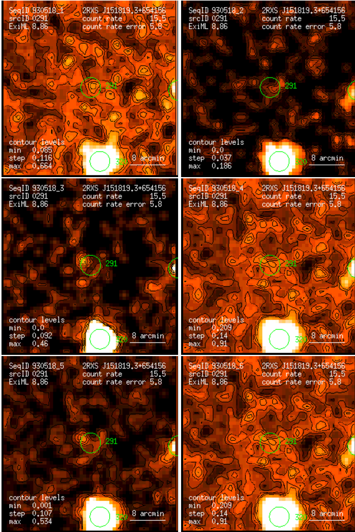
Figure 291: RASS 930518: detection 0291: band rate images, Gaussian filter: (1) PSPC channels 11 – 41, (2) 52 – 90, (3) 91 – 201, (4) 11 – 235, (5) 52 – 201, (6) 11 – 201. Broad band rates in counts/ks. Band rate contour levels in counts/ks/arcmin 2 .
