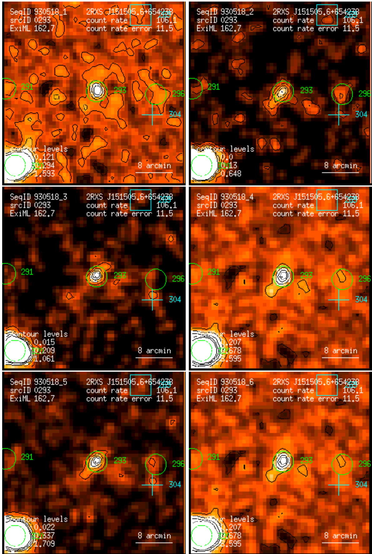
Figure 293: RASS 930518: detection 0293: band rate images, Gaussian filter: (1) PSPC channels 11 – 41, (2) 52 – 90, (3) 91 – 201, (4) 11 – 235, (5) 52 – 201, (6) 11 – 201. Broad band rates in counts/ks. Band rate contour levels in counts/ks/arcmin 2 .
