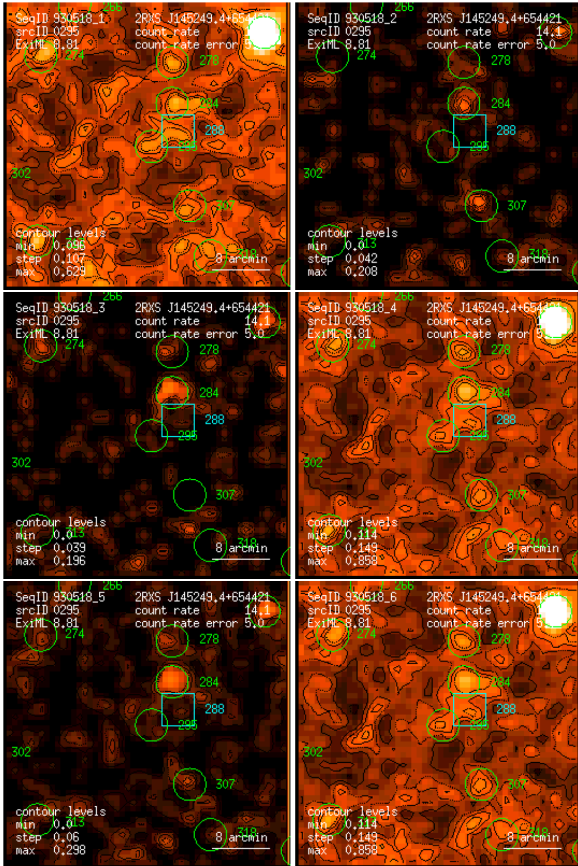
Figure 295: RASS 930518: detection 0295: band rate images, Gaussian filter: (1) PSPC channels 11 – 41, (2) 52 – 90, (3) 91 – 201, (4) 11 – 235, (5) 52 – 201, (6) 11 – 201. Broad band rates in counts/ks. Band rate contour levels in counts/ks/arcmin 2 .
