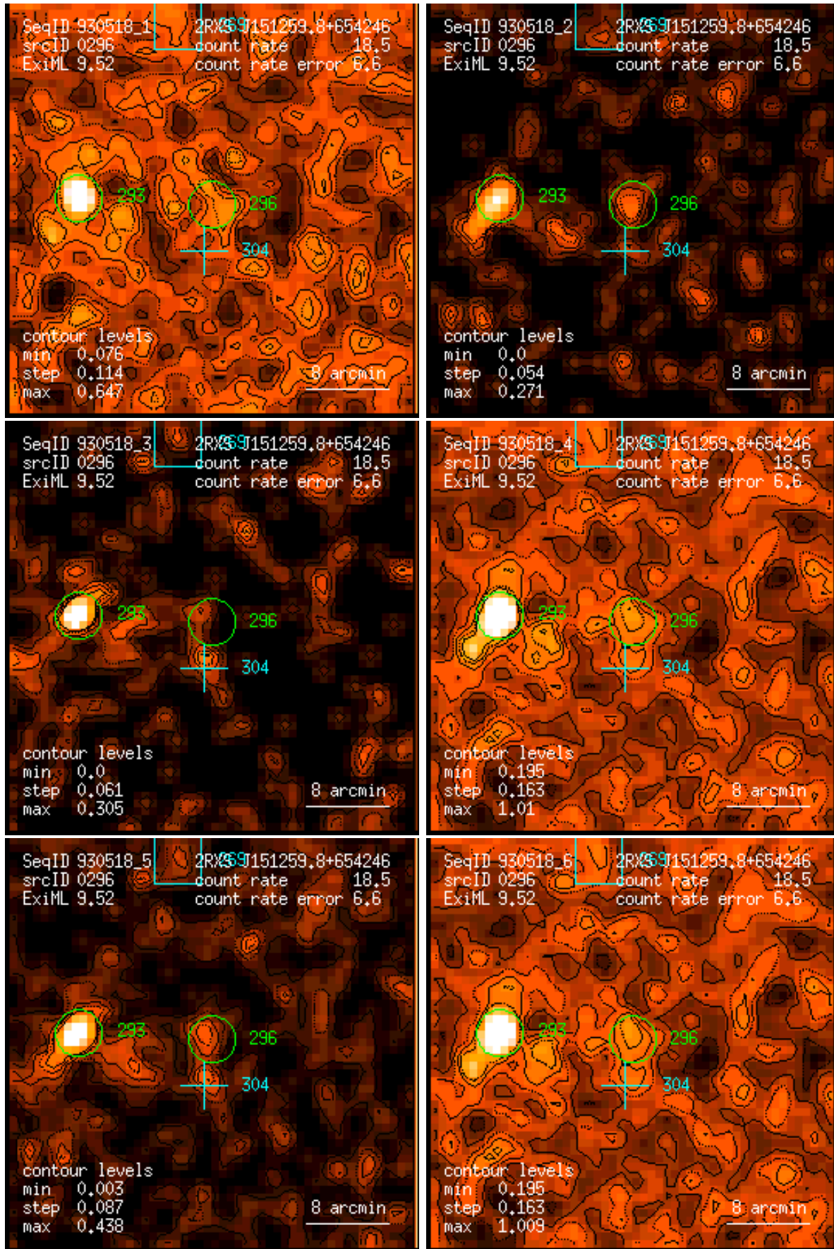
Figure 296: RASS 930518: detection 0296: band rate images, Gaussian filter: (1) PSPC channels 11 – 41, (2) 52 – 90, (3) 91 – 201, (4) 11 – 235, (5) 52 – 201, (6) 11 – 201. Broad band rates in counts/ks. Band rate contour levels in counts/ks/arcmin 2 .
