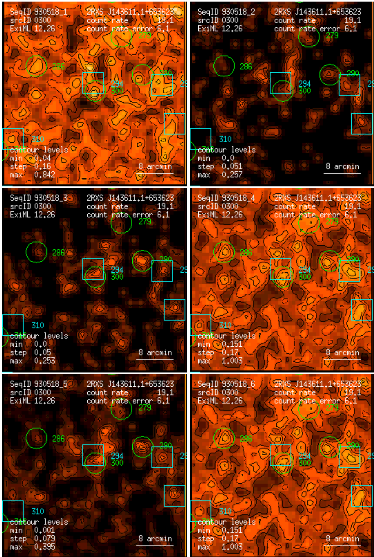
Figure 300: RASS 930518: detection 0300: band rate images, Gaussian filter: (1) PSPC channels 11 – 41, (2) 52 – 90, (3) 91 – 201, (4) 11 – 235, (5) 52 – 201, (6) 11 – 201. Broad band rates in counts/ks. Band rate contour levels in counts/ks/arcmin 2 .
