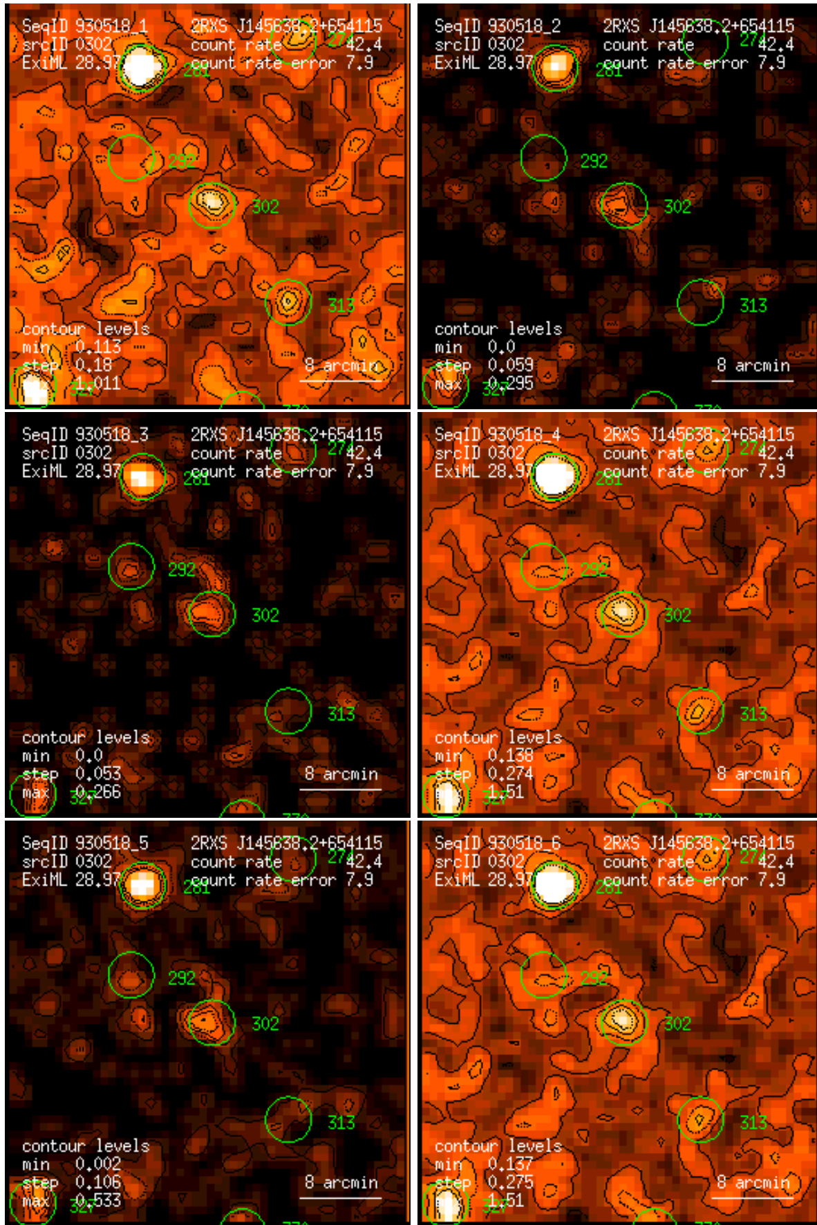
Figure 302: RASS 930518: detection 0302: band rate images, Gaussian filter: (1) PSPC channels 11 – 41, (2) 52 – 90, (3) 91 – 201, (4) 11 – 235, (5) 52 – 201, (6) 11 – 201. Broad band rates in counts/ks. Band rate contour levels in counts/ks/arcmin 2 .
