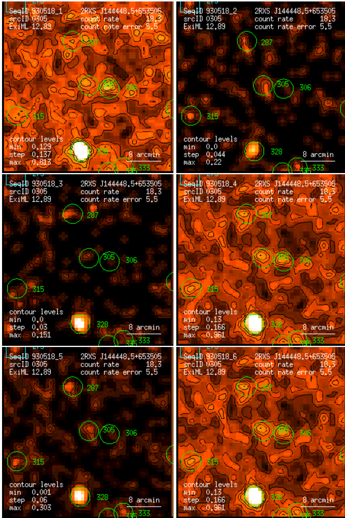
Figure 305: RASS 930518: detection 0305: band rate images, Gaussian filter: (1) PSPC channels 11 – 41, (2) 52 – 90, (3) 91 – 201, (4) 11 – 235, (5) 52 – 201, (6) 11 – 201. Broad band rates in counts/ks. Band rate contour levels in counts/ks/arcmin 2 .
