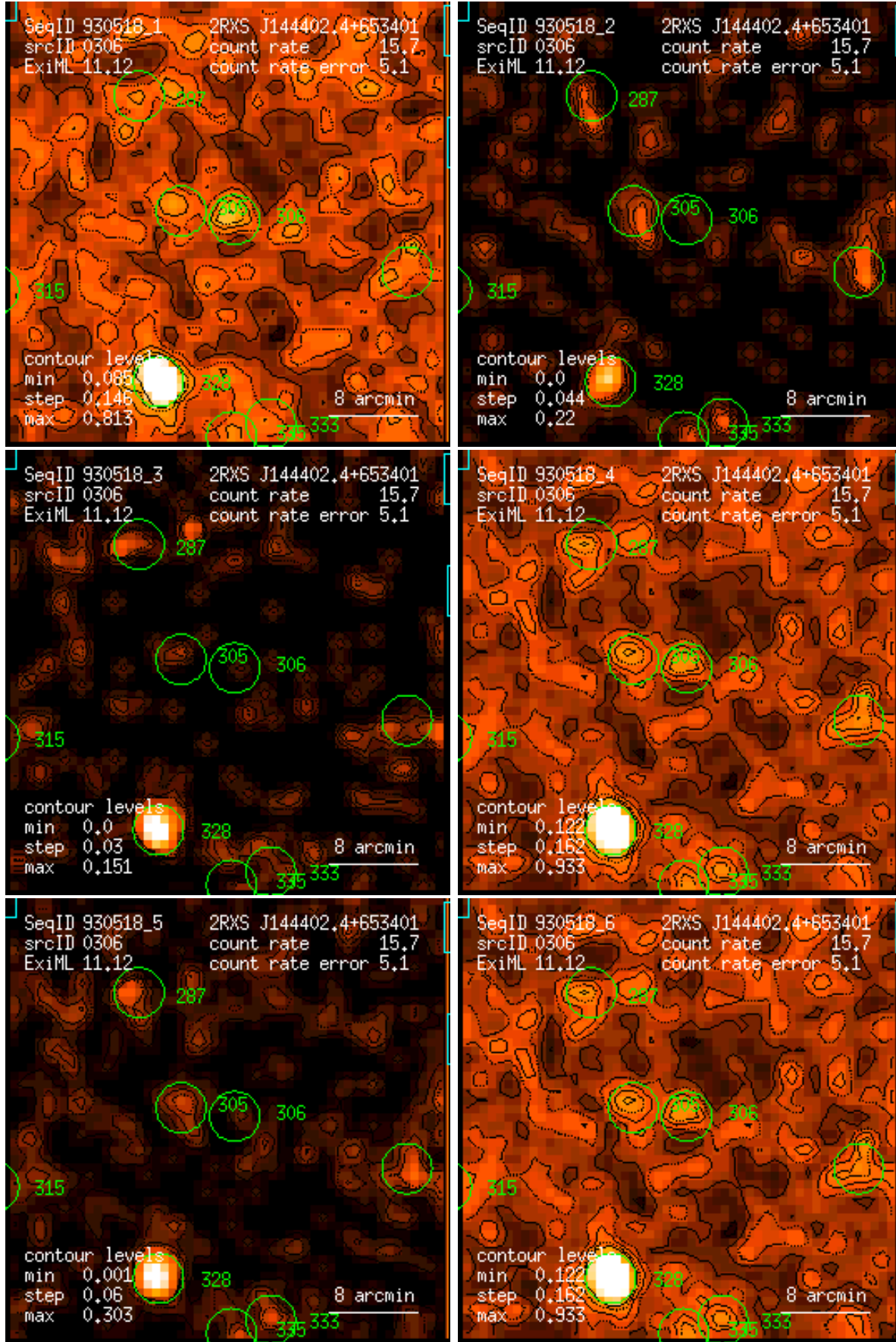
Figure 306: RASS 930518: detection 0306: band rate images, Gaussian filter: (1) PSPC channels 11 – 41, (2) 52 – 90, (3) 91 – 201, (4) 11 – 235, (5) 52 – 201, (6) 11 – 201. Broad band rates in counts/ks. Band rate contour levels in counts/ks/arcmin 2 .
