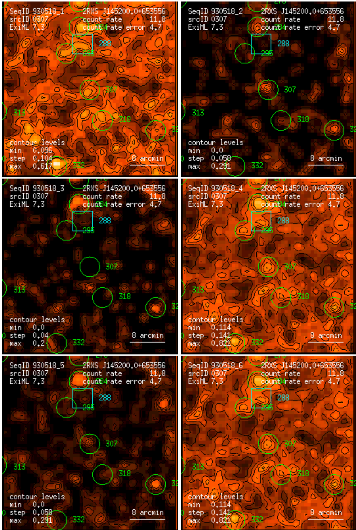
Figure 307: RASS 930518: detection 0307: band rate images, Gaussian filter: (1) PSPC channels 11 – 41, (2) 52 – 90, (3) 91 – 201, (4) 11 – 235, (5) 52 – 201, (6) 11 – 201. Broad band rates in counts/ks. Band rate contour levels in counts/ks/arcmin 2 .
