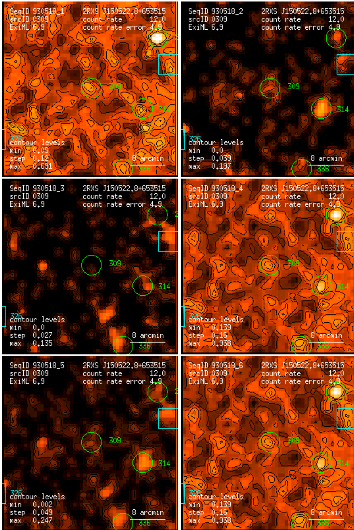
Figure 309: RASS 930518: detection 0309: band rate images, Gaussian filter: (1) PSPC channels 11 – 41, (2) 52 – 90, (3) 91 – 201, (4) 11 – 235, (5) 52 – 201, (6) 11 – 201. Broad band rates in counts/ks. Band rate contour levels in counts/ks/arcmin 2 .
